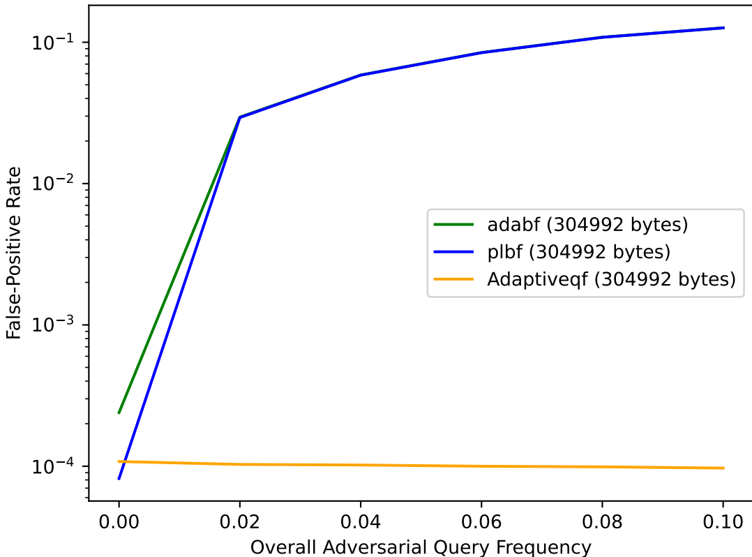
Adversarial Query FPR-Space Tradeoff on url (10.0M Queries)
