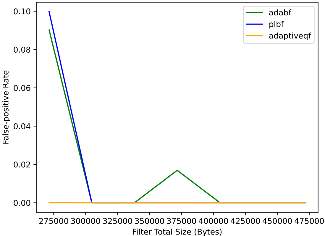
FPR-Space Tradeoff on url (10.0M zipf Queries)
