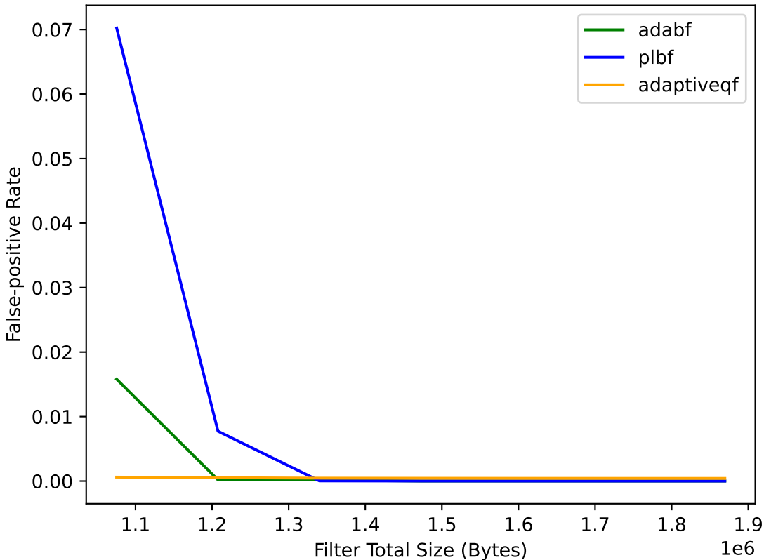
FPR-Space Tradeoff on ember (10.0M zipf Queries)
