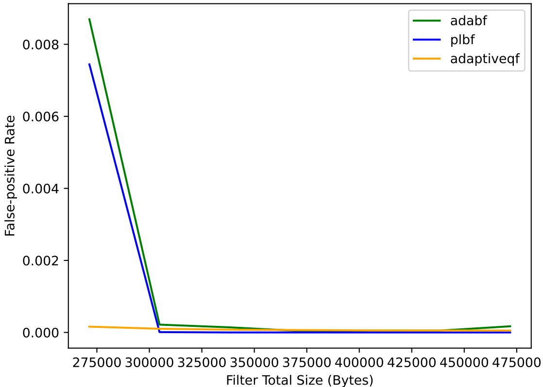
FPR-Space Tradeoff on url (10.0M unif Queries)
