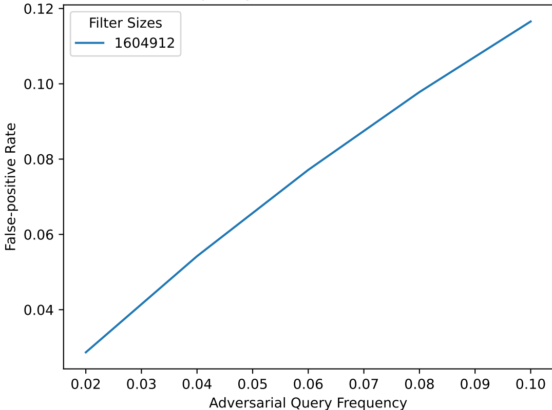
Adversarial Frequency vs FPR (Ember, 10M Queries Total)
