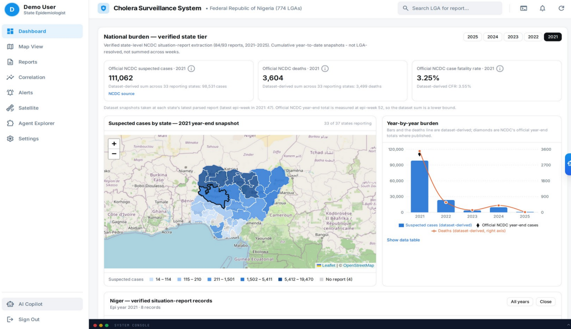
Figure 8b: Verified national tier as deployed — state choropleth of 2021 year-end snapshots (33 reporting states; four states with no parsed report shown as no-data) and the per-state drill-down, here for Niger State, listing every verified record with epi-week, cumulative cases and deaths, CFR, confidence tier, extraction method, monotonicity flag and a link to the exact NCDC situation-report PDF. The dataset-derived national sum (98,531) is displayed as a lower bound beneath the official year-end figure (111,062), never merged with it.
