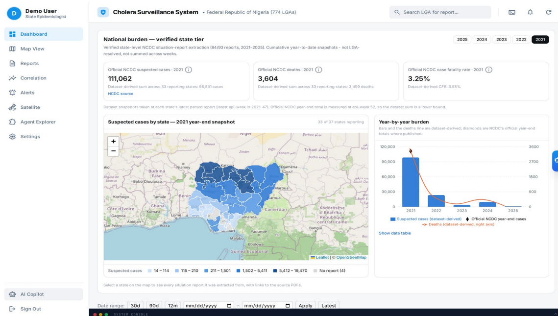
Figure 4: National dashboard as deployed. The upper section is the verified national tier — a state-level choropleth of the NCDC situation-report extraction with the official NCDC year-end figures for 2021 (111,062 suspected cases;
