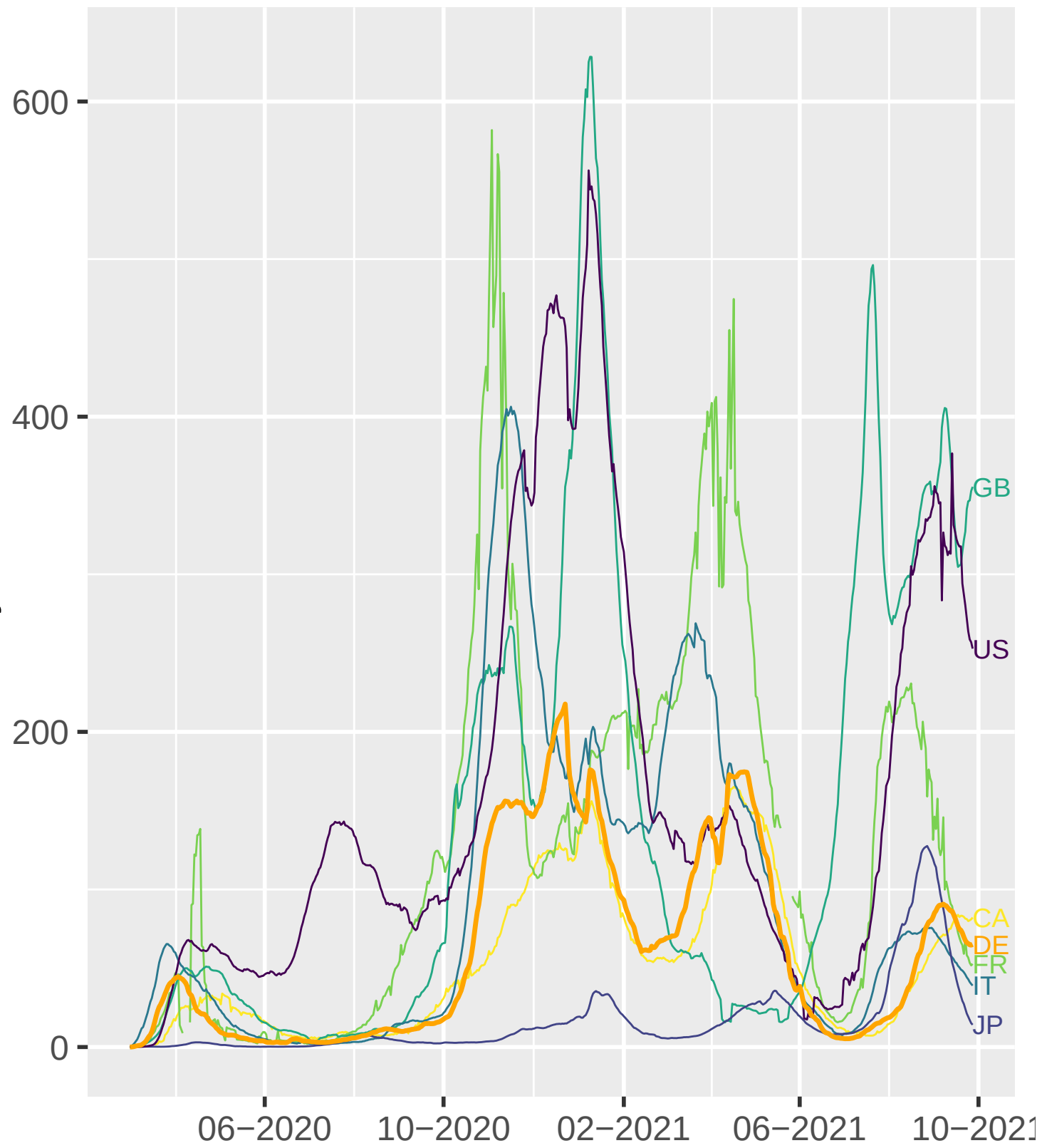
7-Day-Incidence
