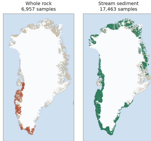
Figure 1: Sample locations after preprocessing. Whole rock is confined to one region of the west coast; stream sediment follows the whole ice-free margin, including the far north and east.
