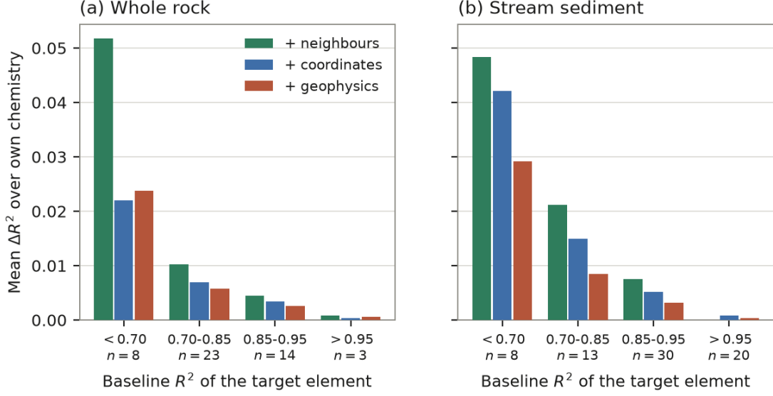
Figure 3: Mean improvement over own chemistry, with targets grouped by how well own chemistry already predicts them. Two datasets with different sampling geometries, different target sets and different element counts produce almost the same curve.
