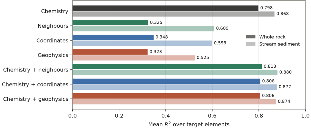
Figure 5: Mean R^2 by feature source, coverage-threshold target sets. Colour identifies the feature source, opacity the dataset. The upper block (spatial information alone) roughly doubles from whole rock to stream sediment; the lower block (the same information on top of own chemistry) barely moves.
