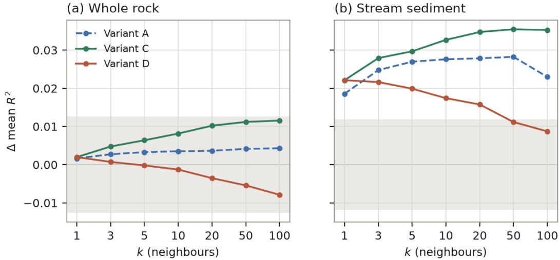
Figure 2: Change in mean R^2 over the no-neighbour baseline as neighbourhood size k varies, on the ten best-covered elements of each dataset. The grey band is one fold standard deviation. Variant C (pooled) rises and plateaus; variant D (enumerated) falls in step with its column count. Absolute levels reflect the ten-element target sets (Section 3.8); the shape is what this figure establishes.
