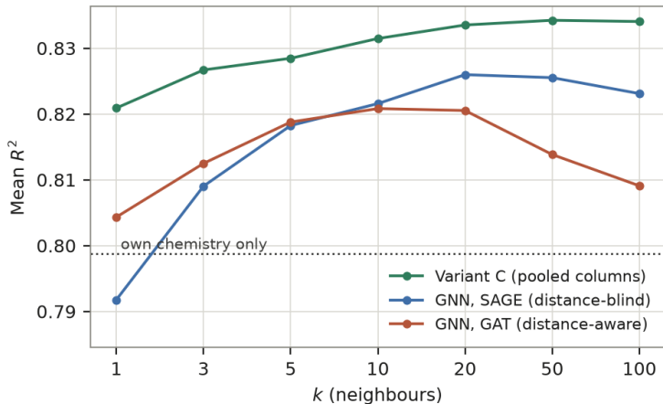
Figure 6: Mean R^2 on stream sediment for the two graph architectures and the hand-built pooled encoding, across neighbourhood size. Variant C dominates both networks at every k . Distance-aware attention (GAT) beats the distance-blind control (SAGE) only below k \approx 5 , and degrades above k = 20 .
