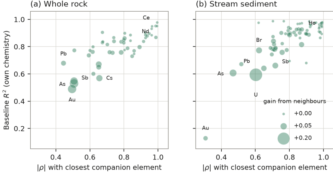
Figure 4: Baseline R^2 against companion strength, one point per target element; marker area is the gain from neighbour features. Elements with a near-perfect companion sit top right and gain nothing; chemically isolated elements sit lower left and are where the neighbourhood pays. Uranium is the extreme case on stream sediment.
