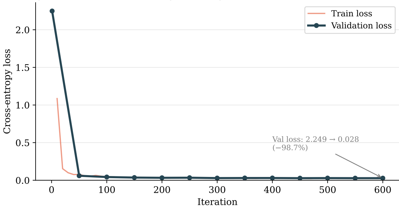
Figure 1: LoRA Fine-tuning Convergence (Qwen2.5-7B, 872 examples)
