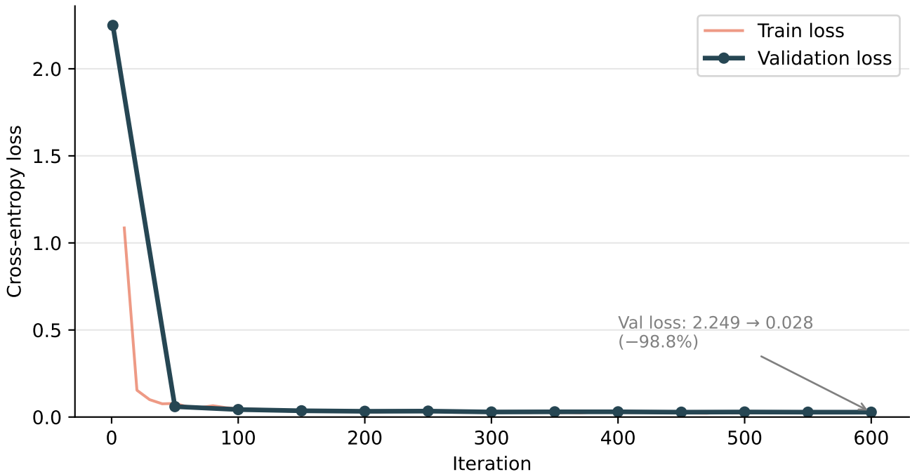
LoRA Fine-tuning Convergence (Qwen2.5-7B, 872 examples)
