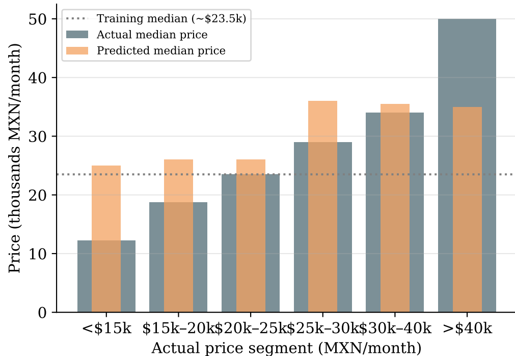
(b) Median Bias Toward Training Distribution
