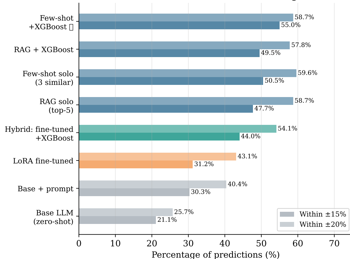
(b) Predictions Within Error Margin
