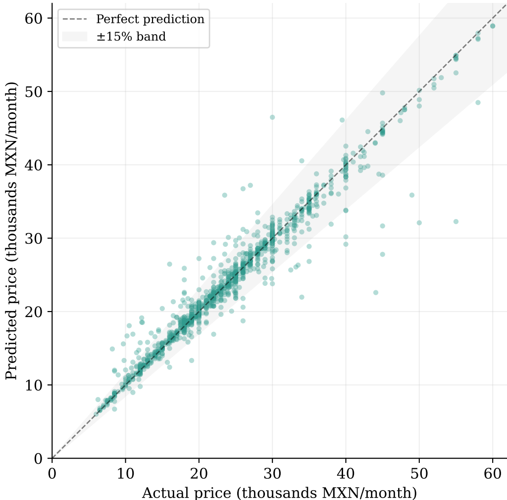
Figure 4: XGBoost Predicted vs. Actual Prices ( R^2=0.70 , MAE= \pm\$3,610 MXN/month)
