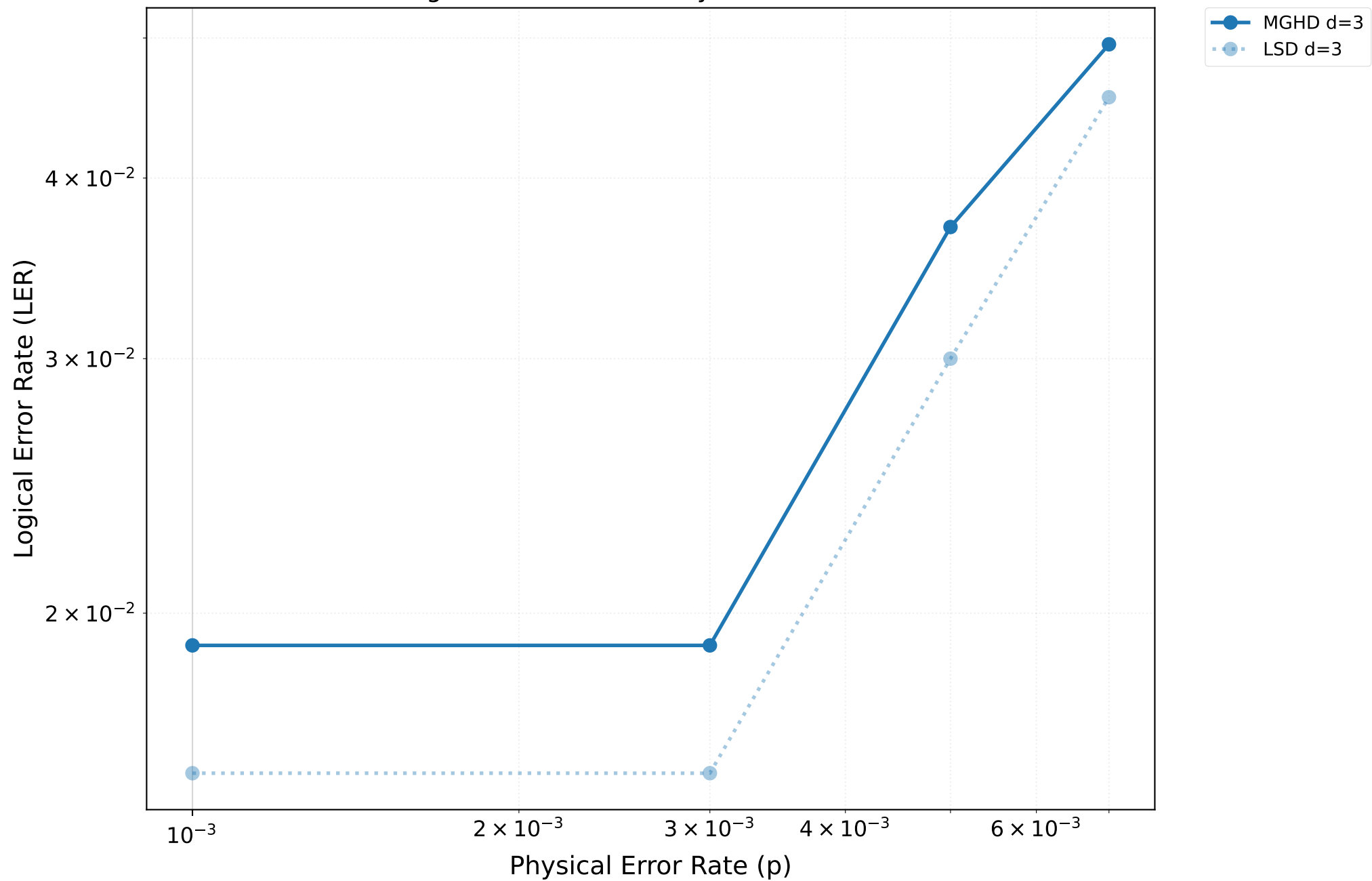
Logical Error Rate vs Physical Error Rate
