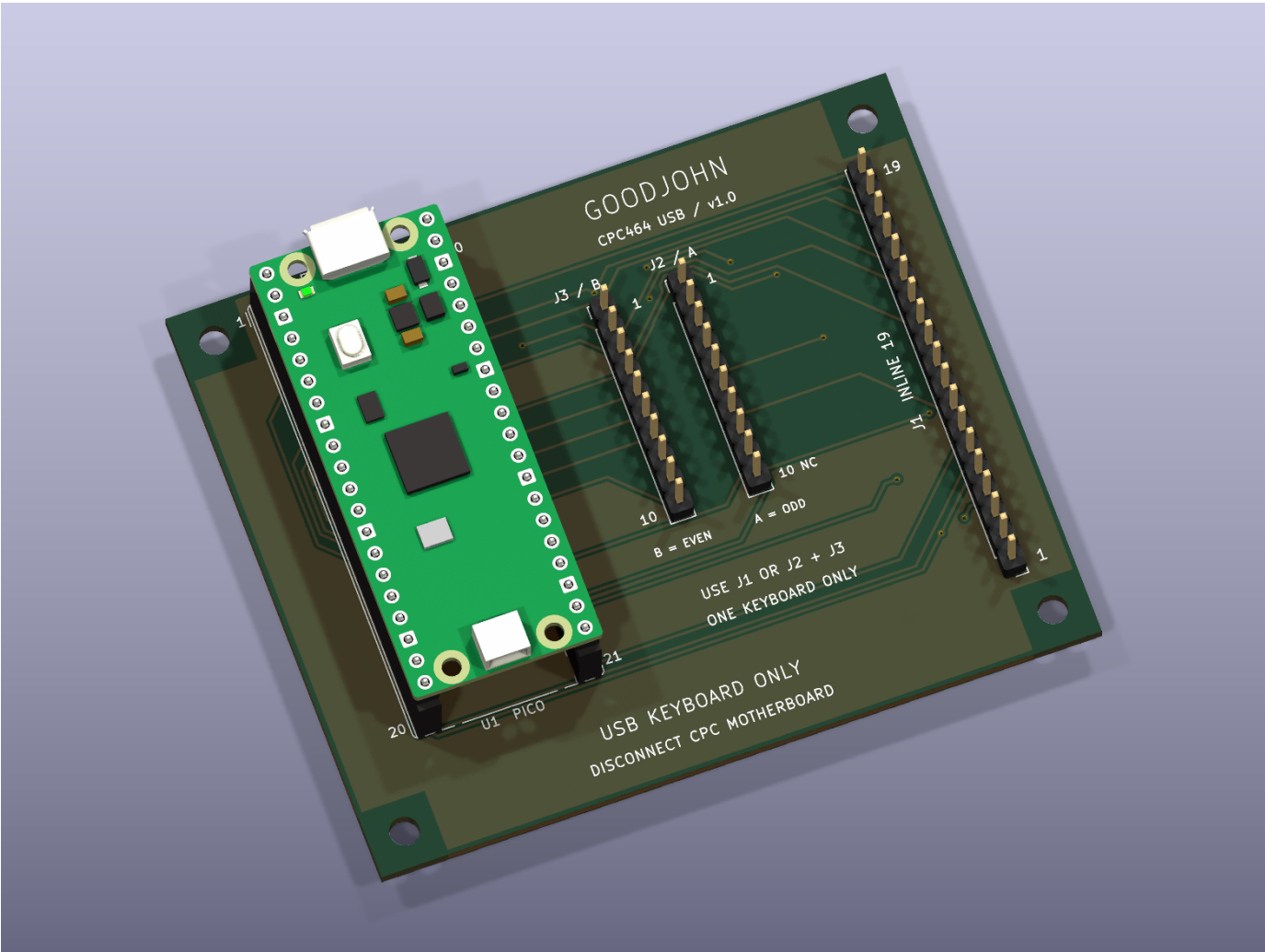
KiCad render; 80 x 66 mm board. Four 3.2 mm mounting holes.
