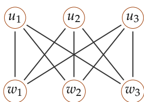
H_1 = K_{3,3}
