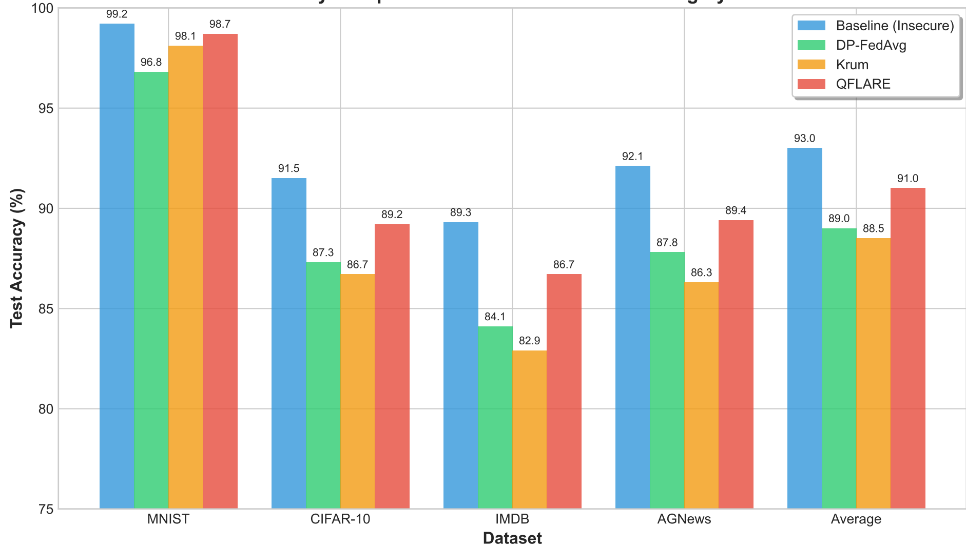
Accuracy Comparison Across Federated Learning Systems
