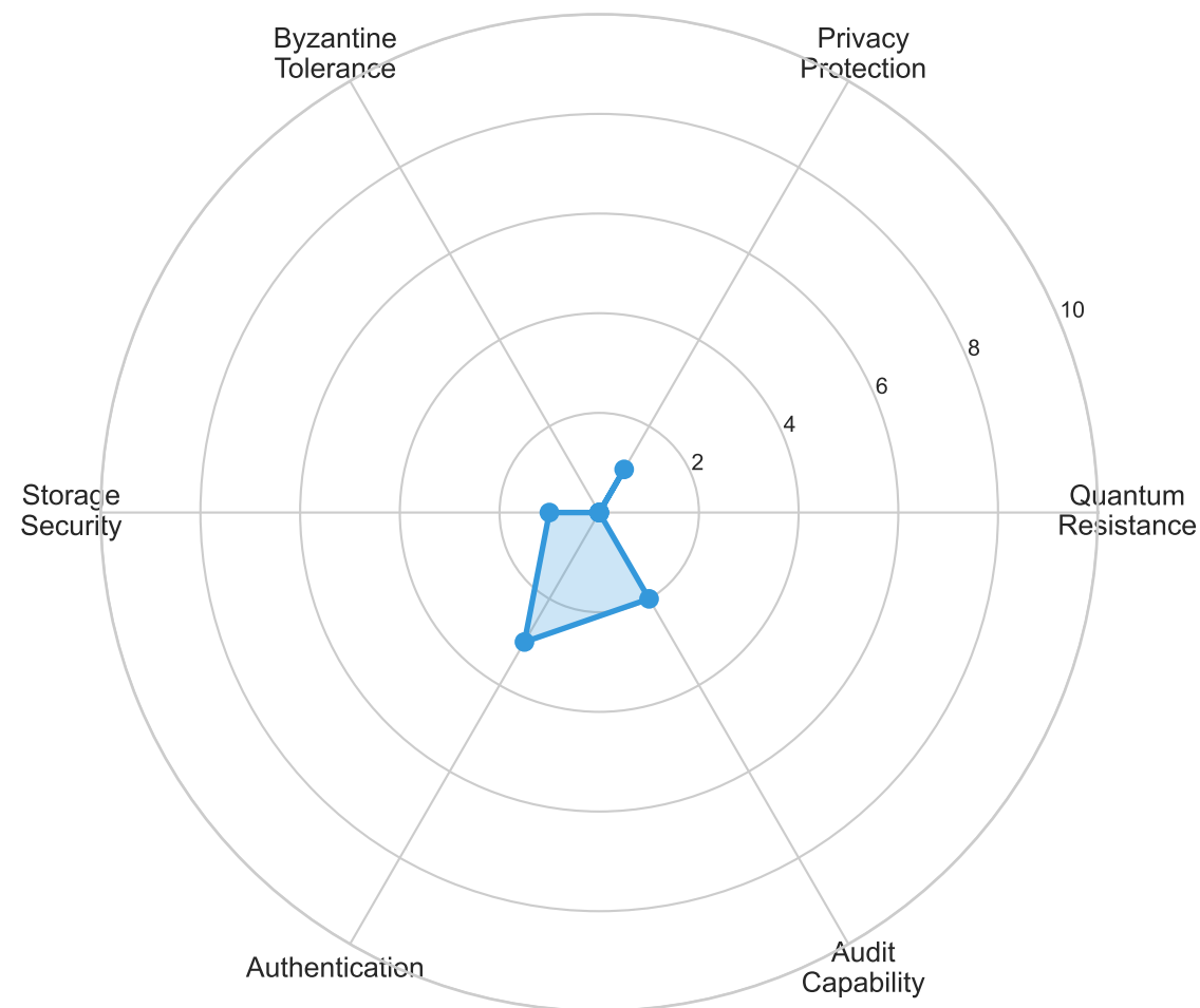
FedAvg
