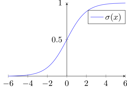
Figure 3: Sigmoid function
