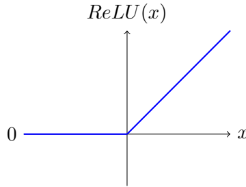
Figure 2: ReLU function
