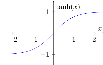
Figure 4: Tanh function
