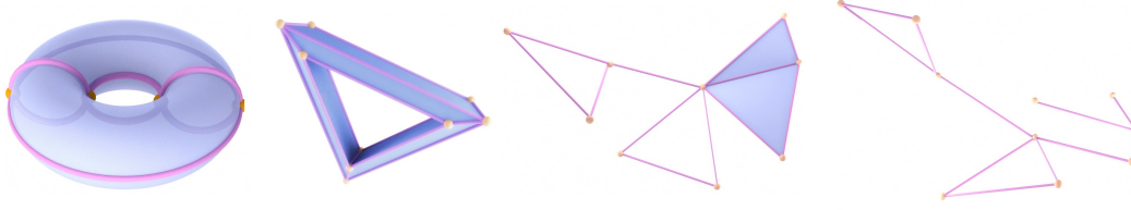
Figure 6: Four examples of regular cell complexes.
