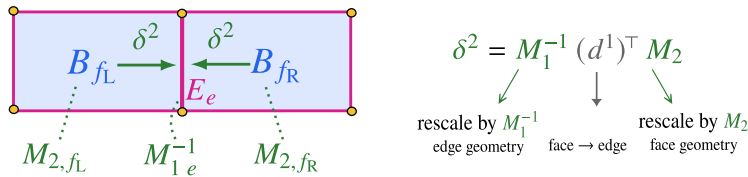
Figure 8: Codifferential as face-to-edge transport. For neighboring faces f_L, f_R \in K_2 sharing an edge e \in K_1 , the codifferential \delta^2 = M_1^{-1} (d^1)^\top M_2 maps face quantities B_{f_L}, B_{f_R} to the edge quantity E_e . Equivalently, its action on an edge is (\delta^2 B)_e = (M_1^{-1})_{ee} \sum_{f \supset e} [f : e] (M_2)_{ff} B_f . The incidence term [f : e] determines which faces touch e and with what orientation, while M_2 and M_1^{-1} inject face and edge geometry.
