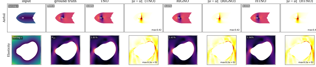
Figure 14: Qualitative comparison on the RIGNO-suite steady-state benchmarks (Airfoil, Elasticity). Each row shows one median-test- L^1 sample for the dataset; columns: input forcing, ground-truth field, and per-architecture prediction \hat{u} followed by absolute error |\hat{u} - u| for TNO, RIGNO, and HTNO. The three error panels in a row share a common color scale, with the shared max stamped on each panel so residual magnitudes are directly comparable across architectures.
