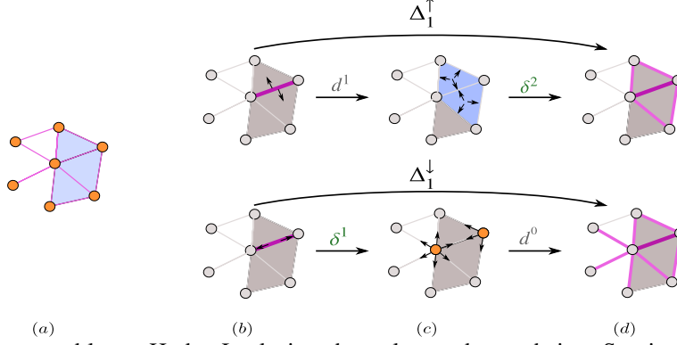
Figure 9: Upper and lower Hodge-Laplacian channels on edge cochains. Starting from an edge-supported signal in C^1(K) , the upper channel first applies d^1 : C^1(K) \rightarrow C^2(K) to accumulate circulation on incident faces and then applies \delta^2 : C^2(K) \rightarrow C^1(K) to return the result to edges, giving \Delta_1^\uparrow = \delta^2 d^1 . This propagates information between edges through shared faces. The lower channel first applies \delta^1 : C^1(K) \rightarrow C^0(K) to aggregate edge information to vertices and then applies d^0 : C^0(K) \rightarrow C^1(K) to return it to edges, giving \Delta_1^\downarrow = d^0 \delta^1 . This propagates information between edges through shared vertices. Together, \Delta_1 = \Delta_1^\uparrow + \Delta_1^\downarrow decomposes same-rank edge propagation into face-mediated and vertex-mediated components.
