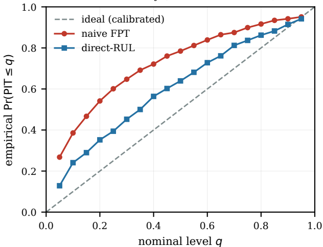
PIT reliability (matched threshold)
