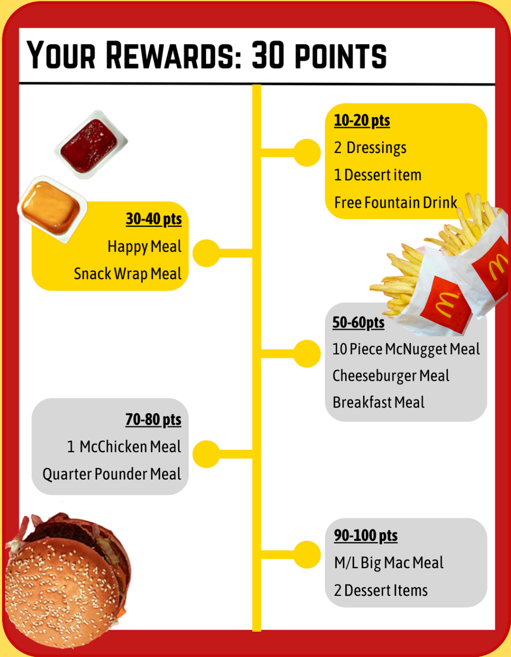
REWARD SYSTEM
