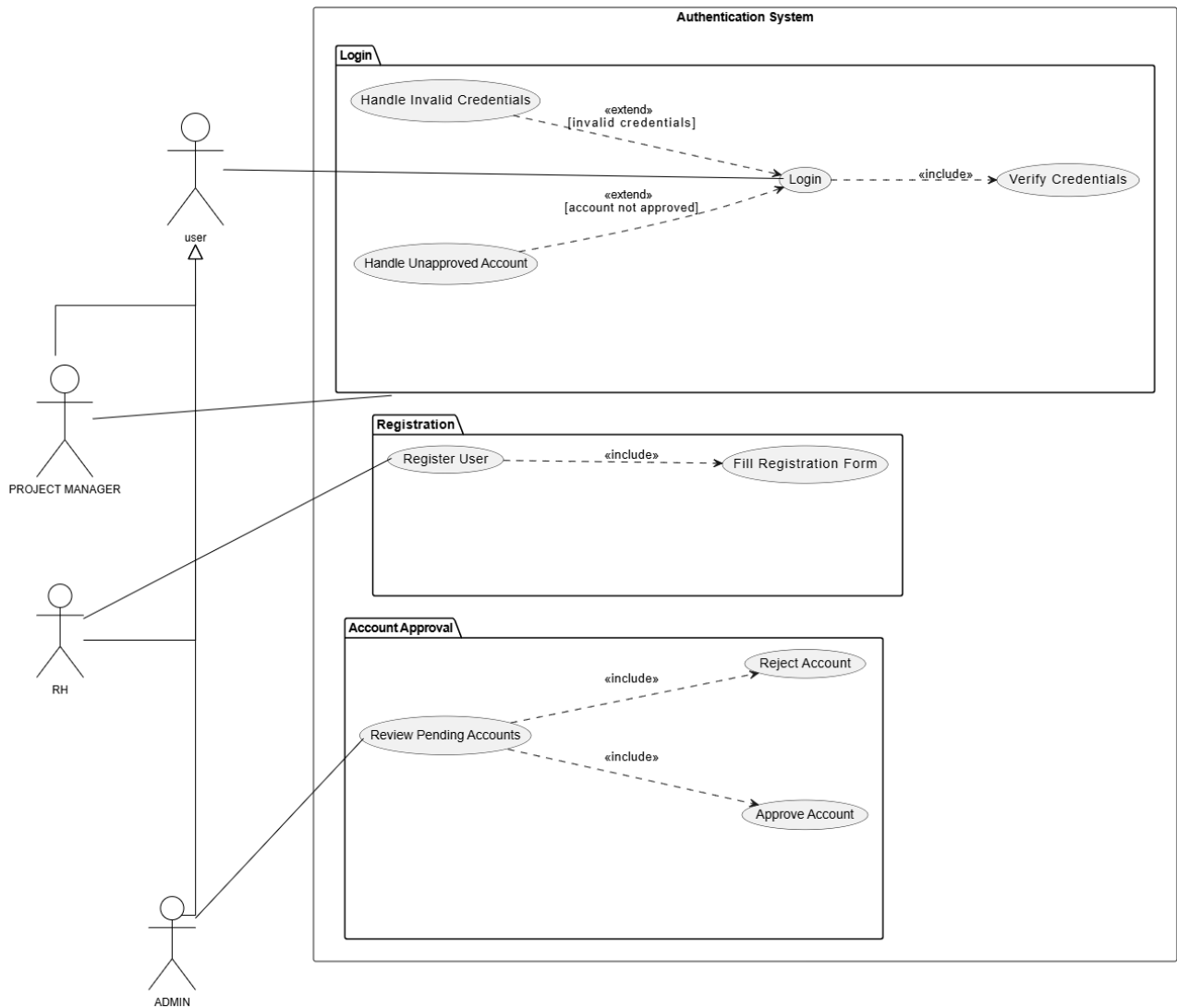
Figure 4.1: Refined use case diagram for authentication and access control
