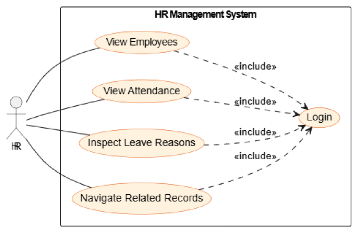
Figure 6.4: HR Employee Attendance and Leave Monitoring Use Case Diagram
