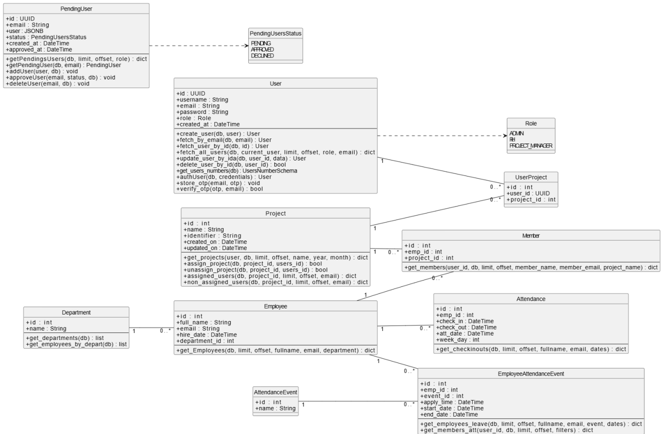
Figure 2.5: Class Diagram
