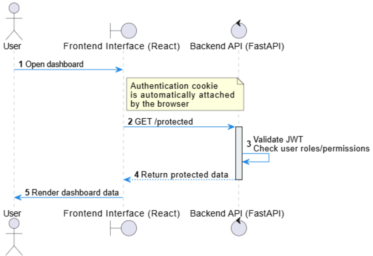
Figure 4.3: Protected route access with JWT verification
