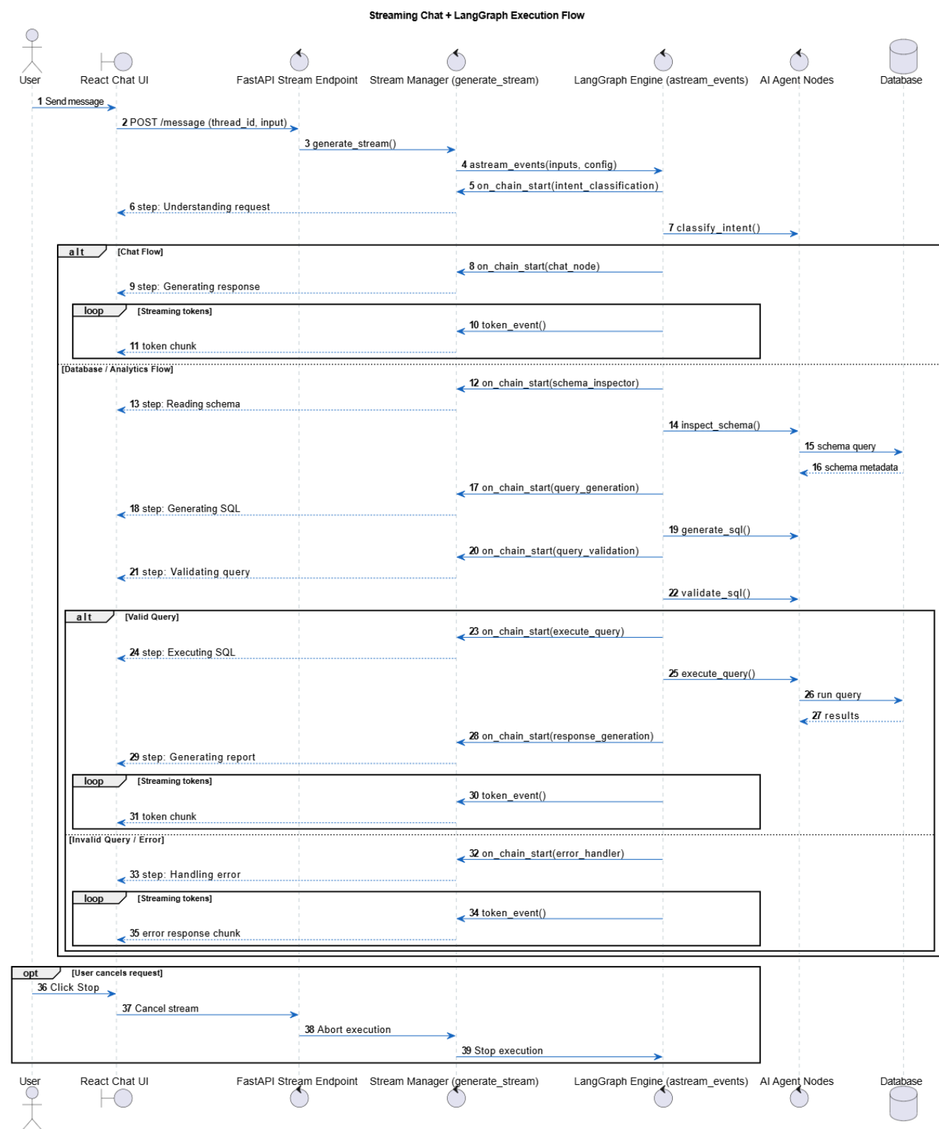
Figure 8.2: Sequence diagram of the RH Agent workflow
