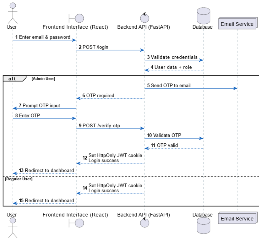
Figure 4.2: Login flow showing JWT token issuance
