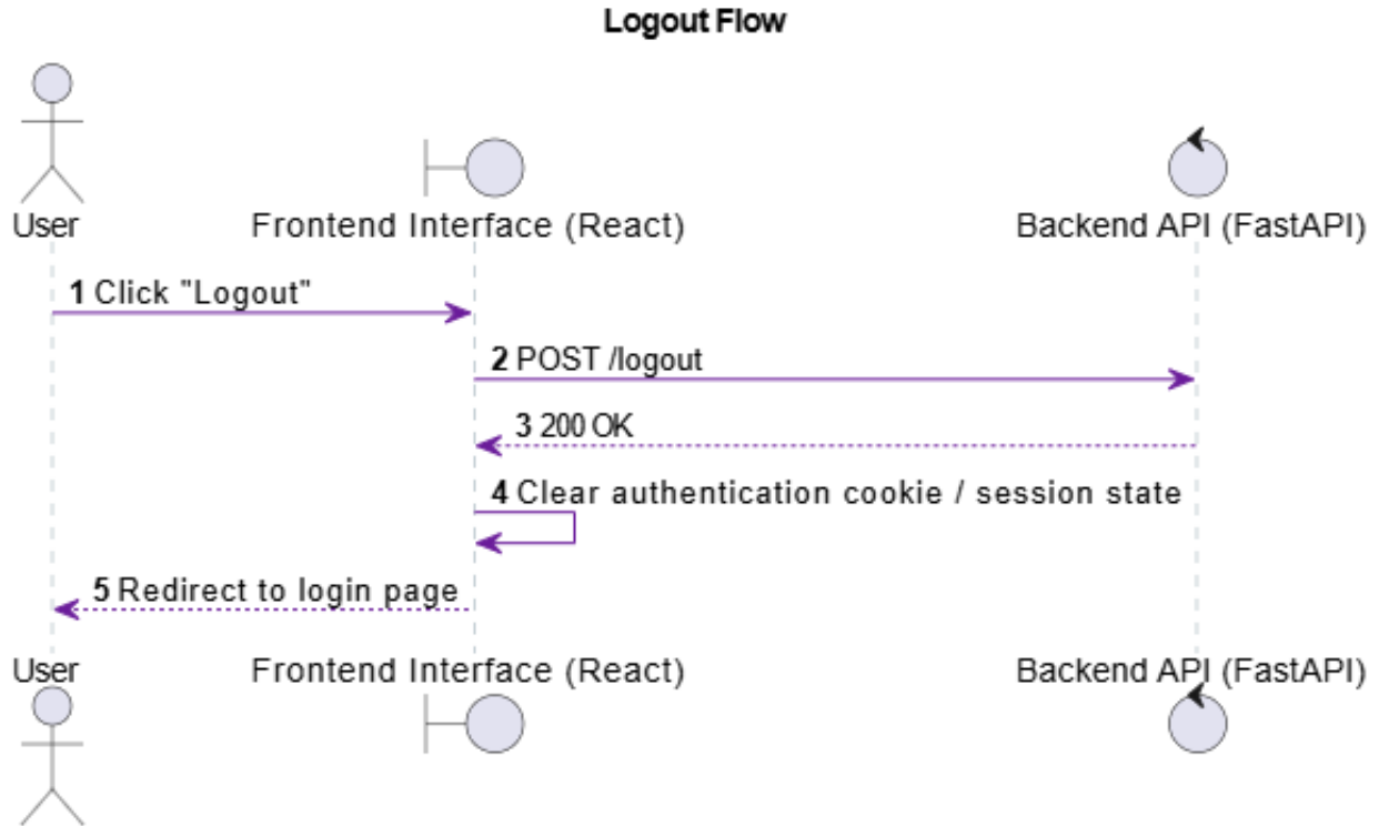
Figure 4.5: Logout flow with token invalidation
