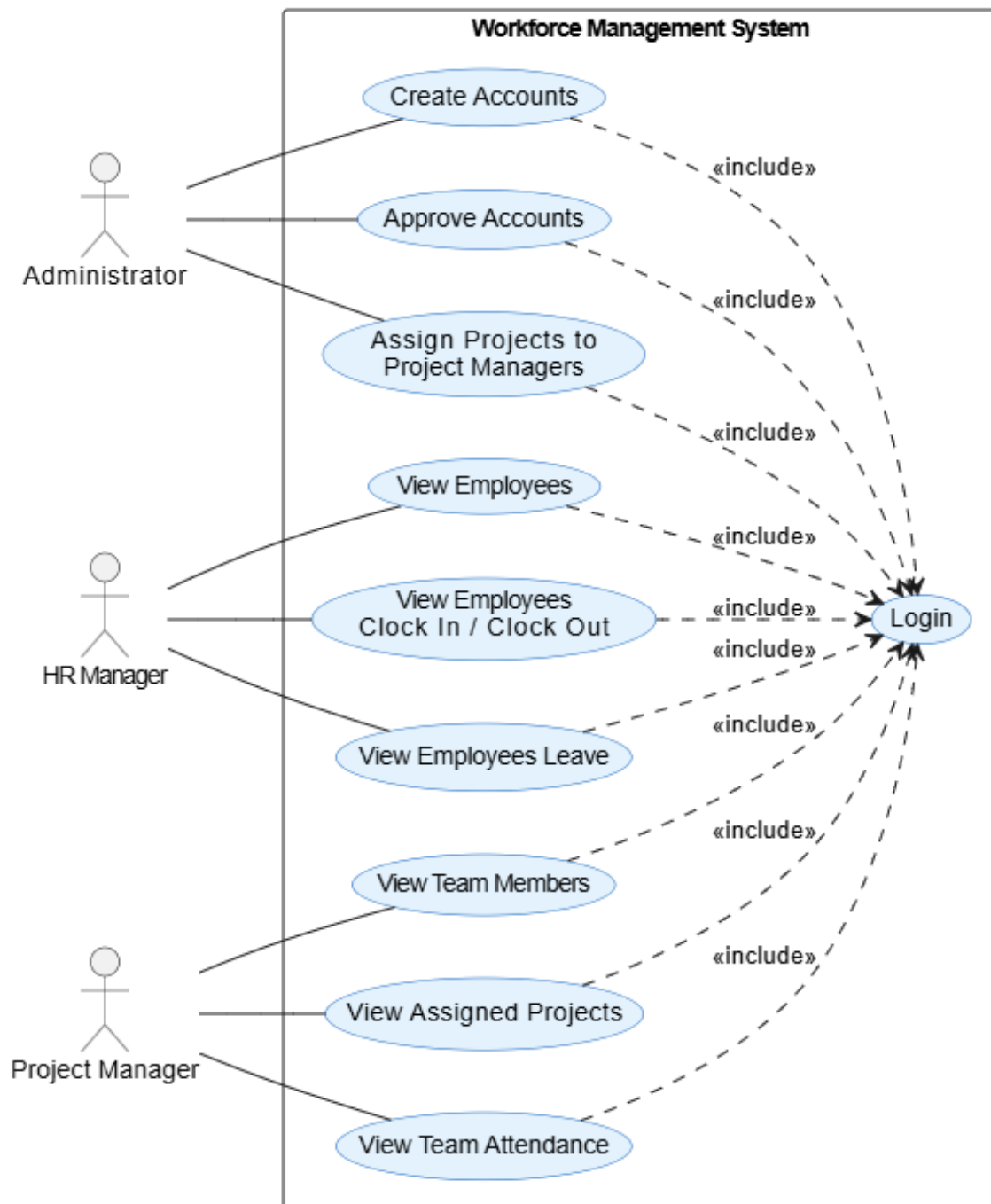
Figure 2.2: Global Use Case Diagram
