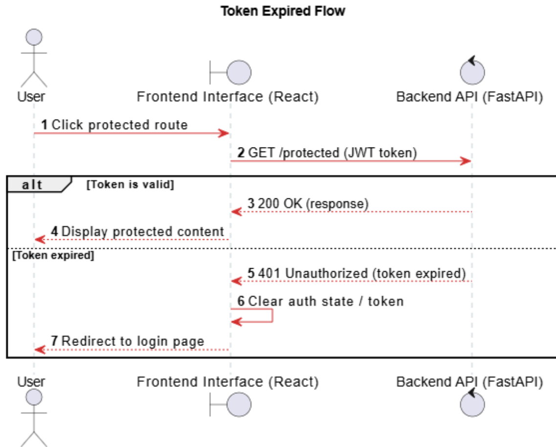
Figure 4.4: Token expiration and re-authentication flow
