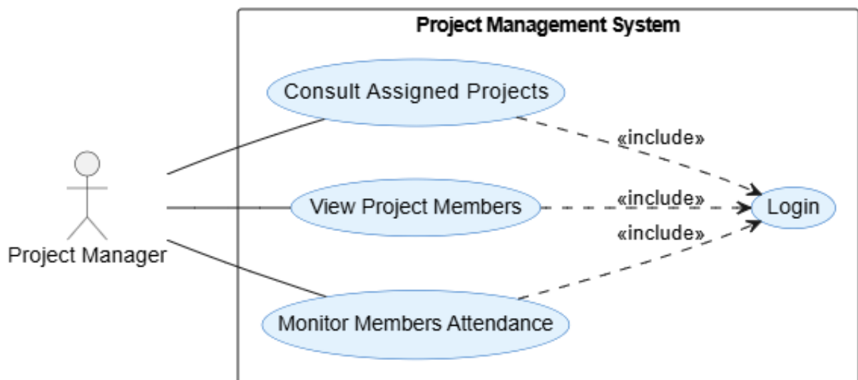
Figure 7.4: Project Manager Supervision and Attendance Monitoring Use Case Diagram
