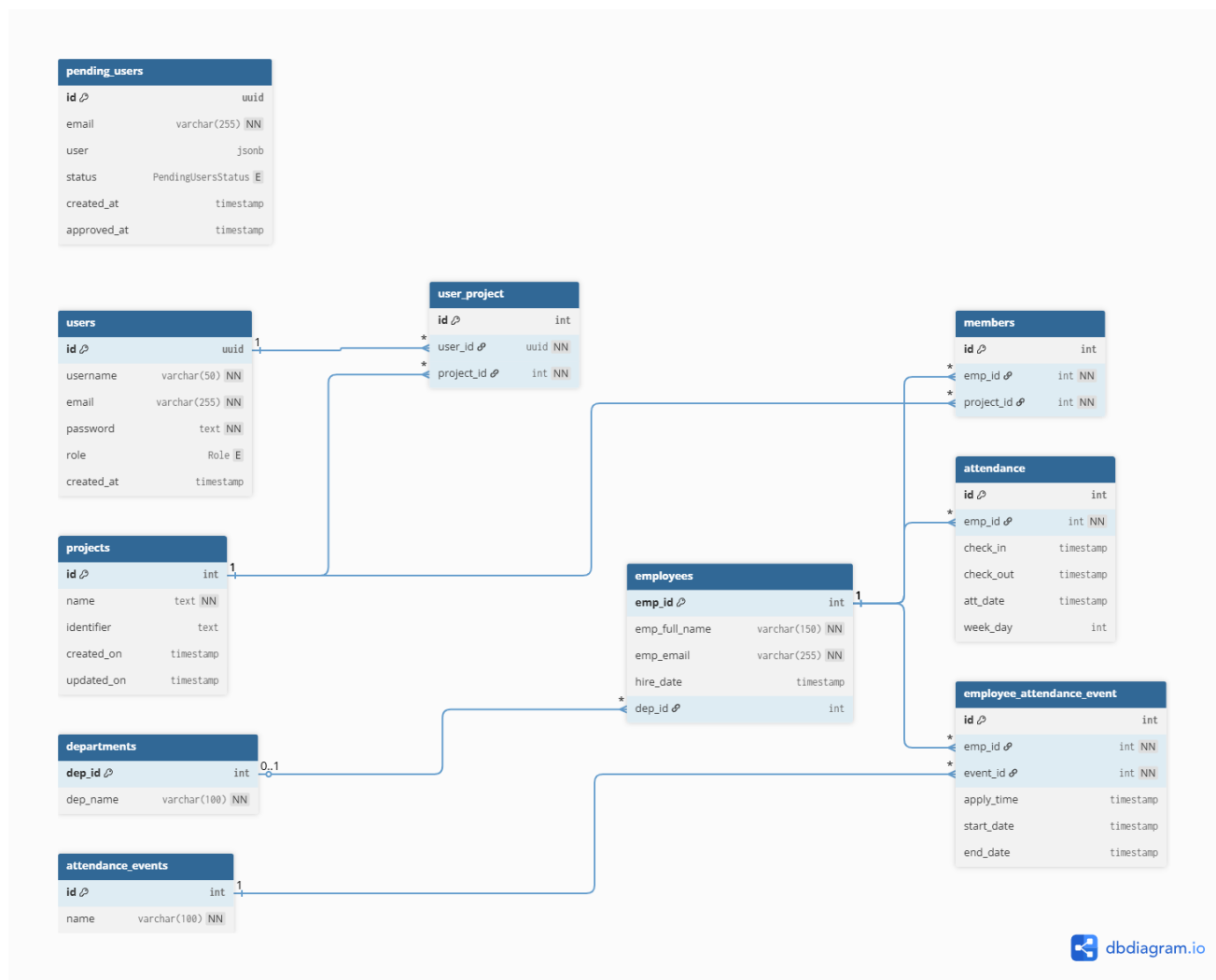
Figure 2.6: Main Application Diagram
