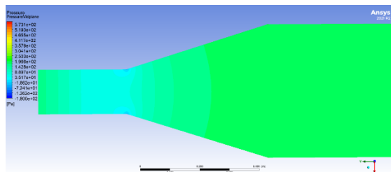
Figure 5.8: Timestep 25 - Uniform Pressure Recovery
