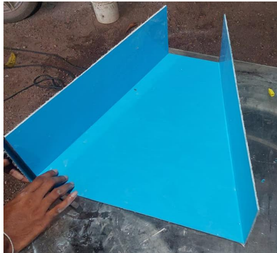
Figure 5.29 - Wide angle diffuser fabrication
