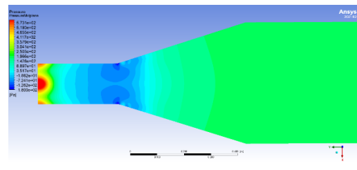
Figure 5.9: Timestep 150 - Early pressure disturbance
