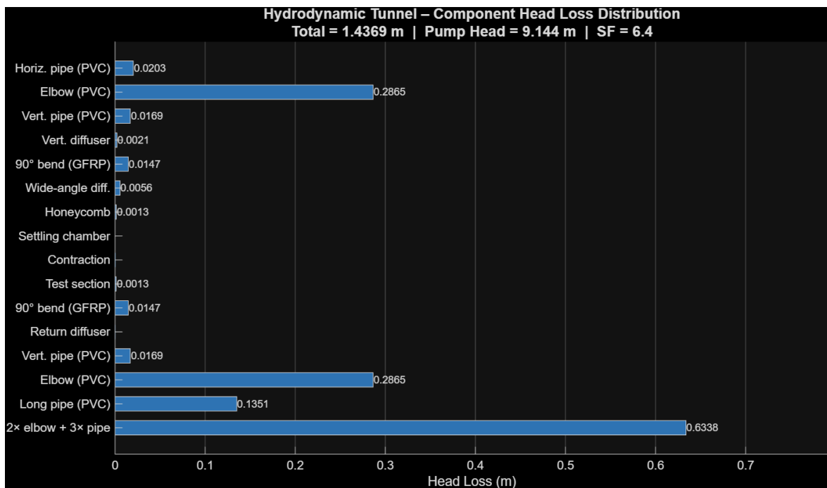
Figure 5.2: Bar chart of component head loss contributions from MATLAB output
