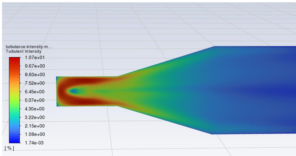
Figure 5.14 - Turbulence intensity decay through the wide-angle diffuser
