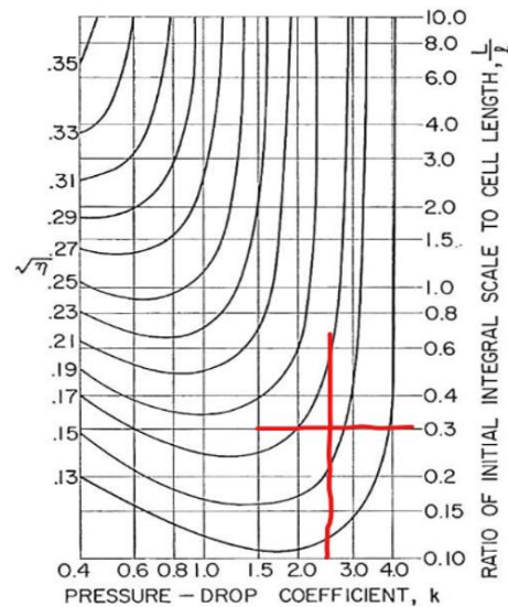
Figure 3.5 : Iso-reduction contours showing the relationship between pressure-drop coefficient and the ratio of the integral length scale of initial turbulence to the cell length [8]
