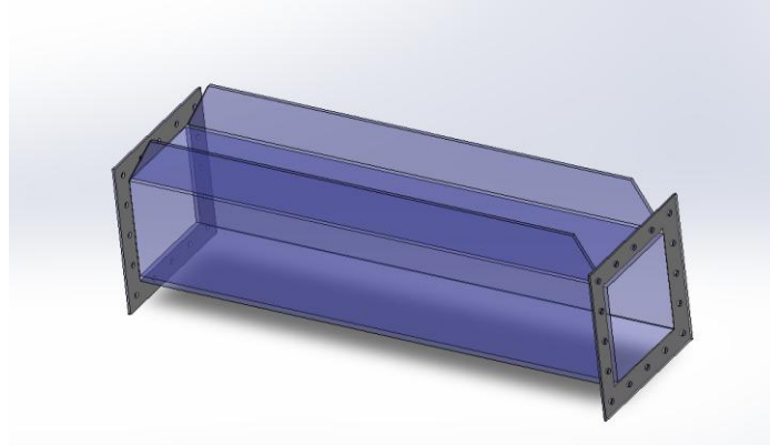
Figure 4.19: Test section detailed drawing
