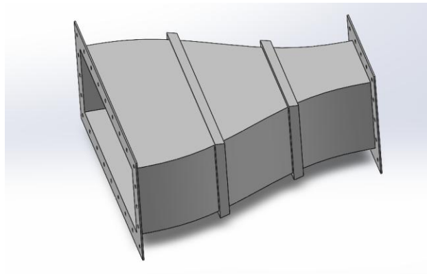
Figure 4.18: Contraction section detailed design
