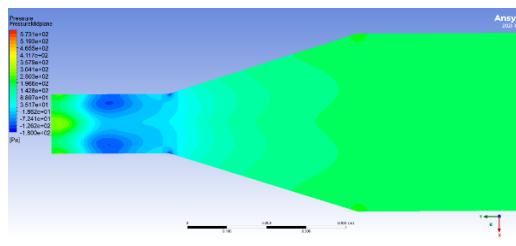
Figure 5.11: Timestep 1960 - Nearly stable pressure distribution
