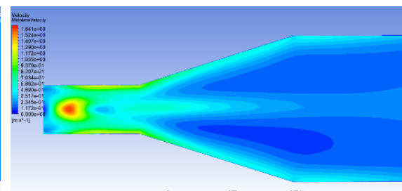
Figure 5.7: Timestep 19.6 S– Quasi steady flow
