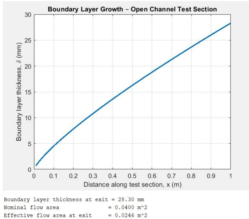
Figure 3.2: Boundary layer growth graph of open channel test section using MATLAB
