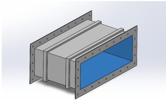
Figure 4.17: Settling chamber
