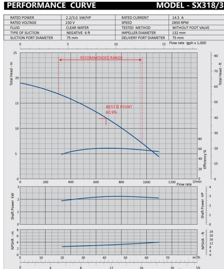
Figure 5.3: SOLEX SX318/3T pump performance characteristic curve
