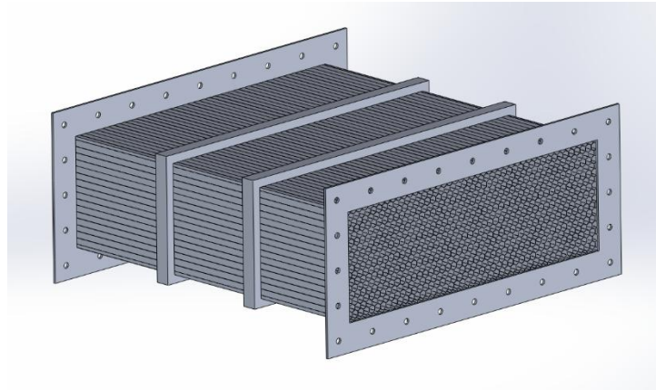
Figure 4.16: Honeycomb structure
