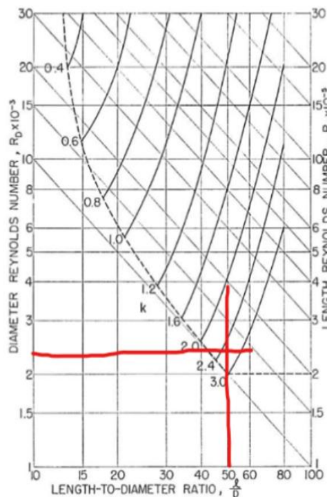
Figure 3.4: Variation of pressure-drop coefficient and length Reynolds number as a function of diameter Reynolds number and length-to-diameter ratio, indicating fully developed flow region above and to the right of the dashed line. The pressure loss across the honeycomb [8]
