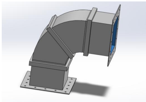
Figure 4.14: Rectangular 90-degree bend
