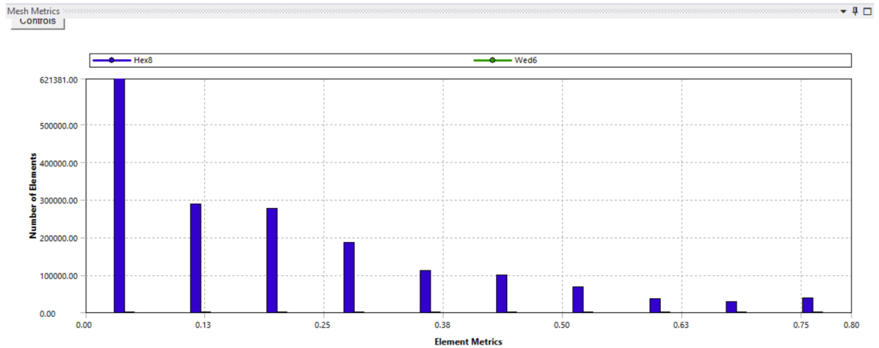
Figure 4.4 – Skewness
