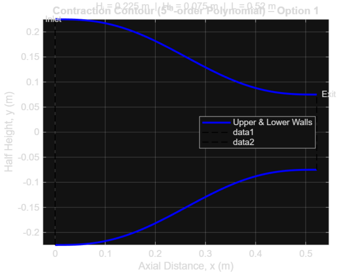
Figure 5.1: Bell-Mehta contraction wall profile plot from MATLAB
