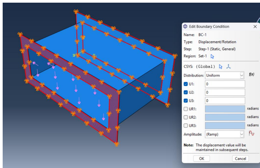
Figure 4.11: Boundary conditions - settling chamber (other components are also like this)
