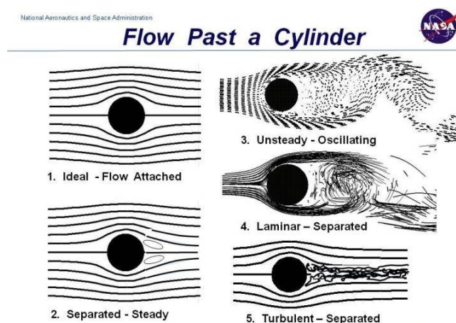
Figure 1.1: flow pattern progression over circular cylinder
