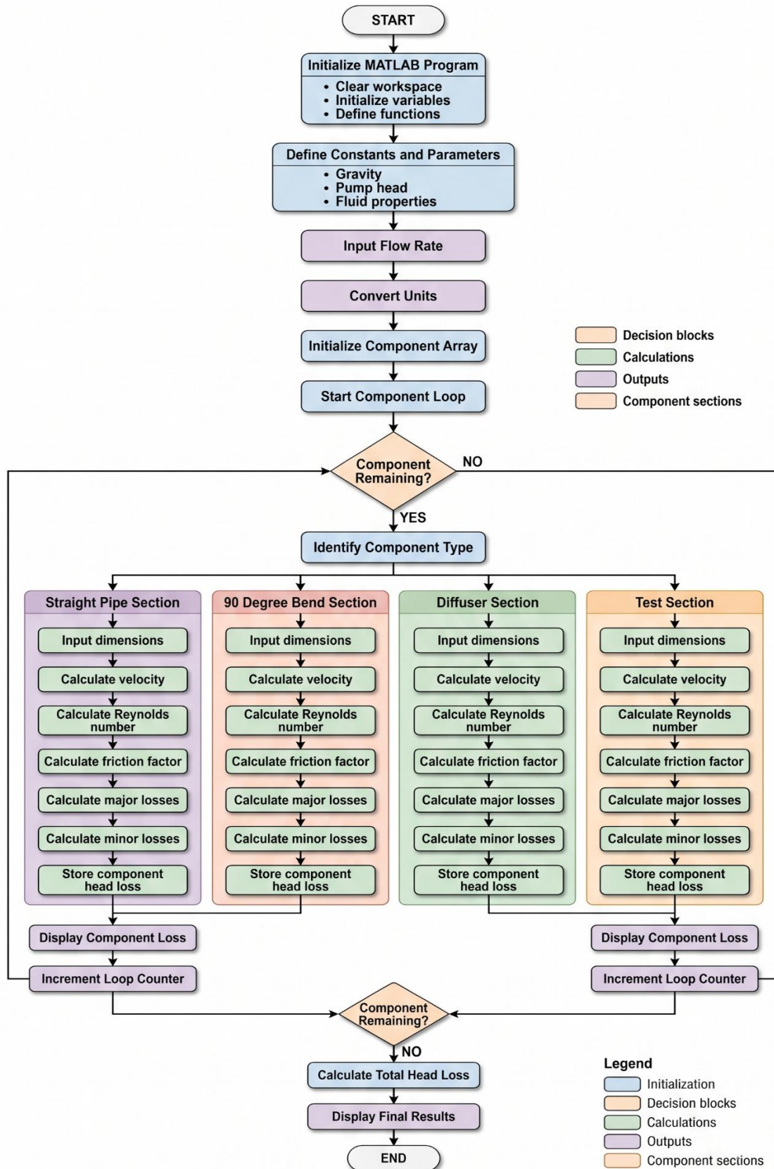
Figure 3.8: Flowchart of the MATLAB head loss model
