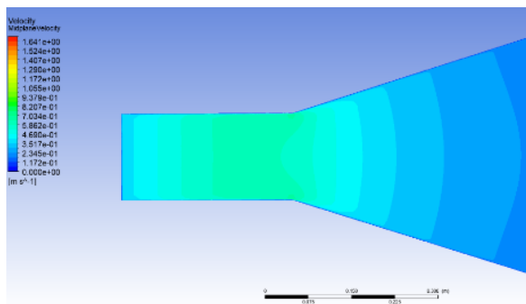
Figure 5.4: 0.25 S - Early transient stage (Attached flow)
