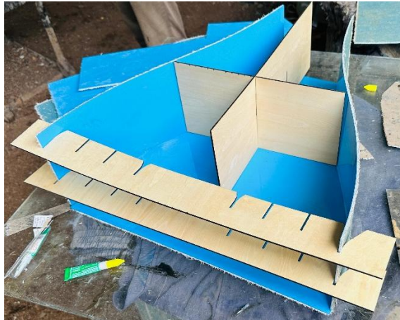
Figure 5.31- Plywood templates used to maintain curved contraction profile during assembly
