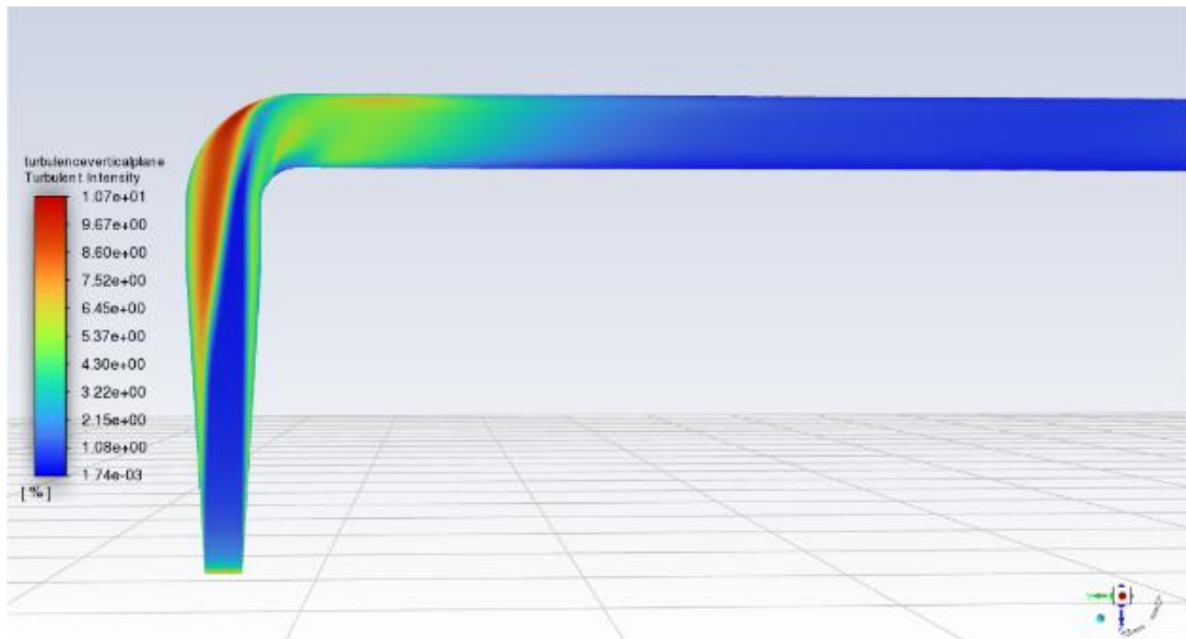
Figure 5.12 - Turbulence intensity variation from diffuser inlet
