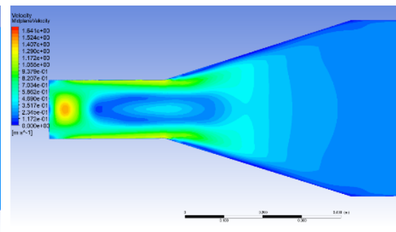
Figure 5.5: 1.5 S – Separation forming
