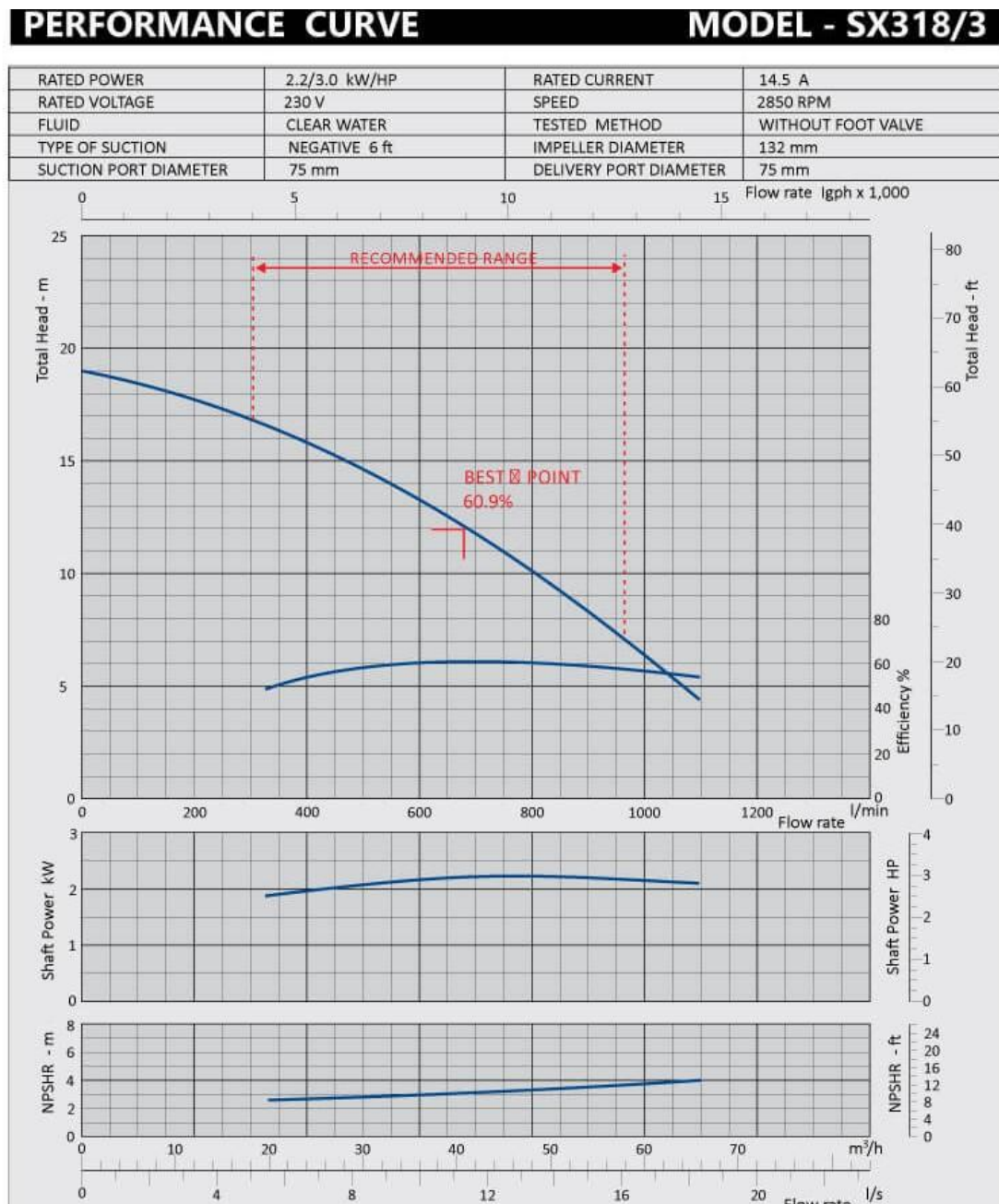
Figure 3.7: Pump characteristic curve
