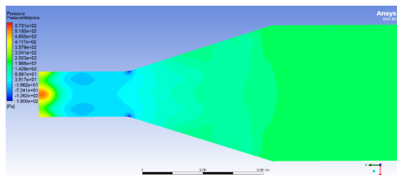
Figure 5.10: Timestep 220 - Symmetric Low-Pressure Regions
