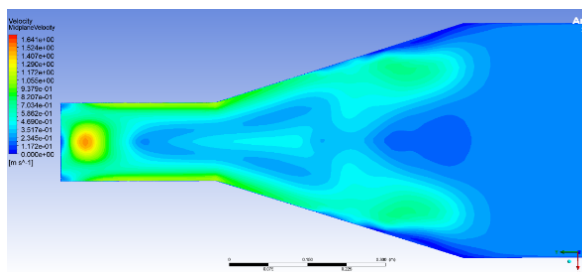
Figure 5.6: 2.2 S - Developed separation
