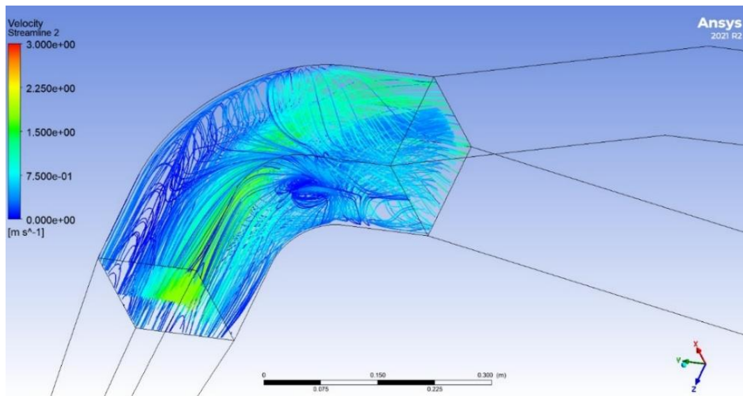
Figure 5.13 - 90 bend Velocity streamlines
