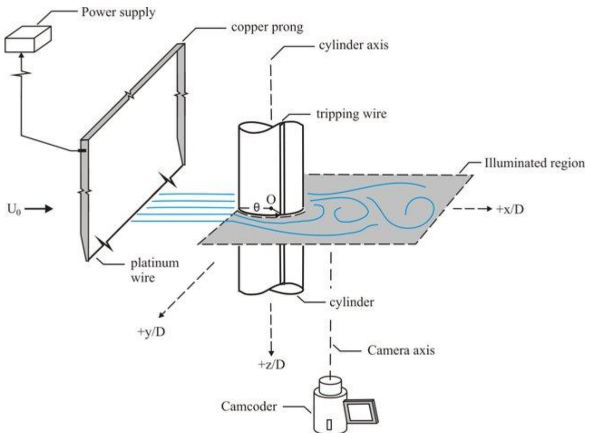
Figure 3.9: A representative schematic of the experimental setup employing the hydrogen bubble flow visualization system. The cylinder/wire and the platinum wire holder
