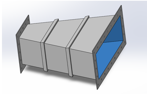
Figure 4.15: Wide angle diffuser
