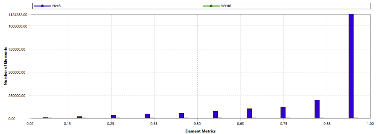
Figure 4.5 - Orthogonal quality
