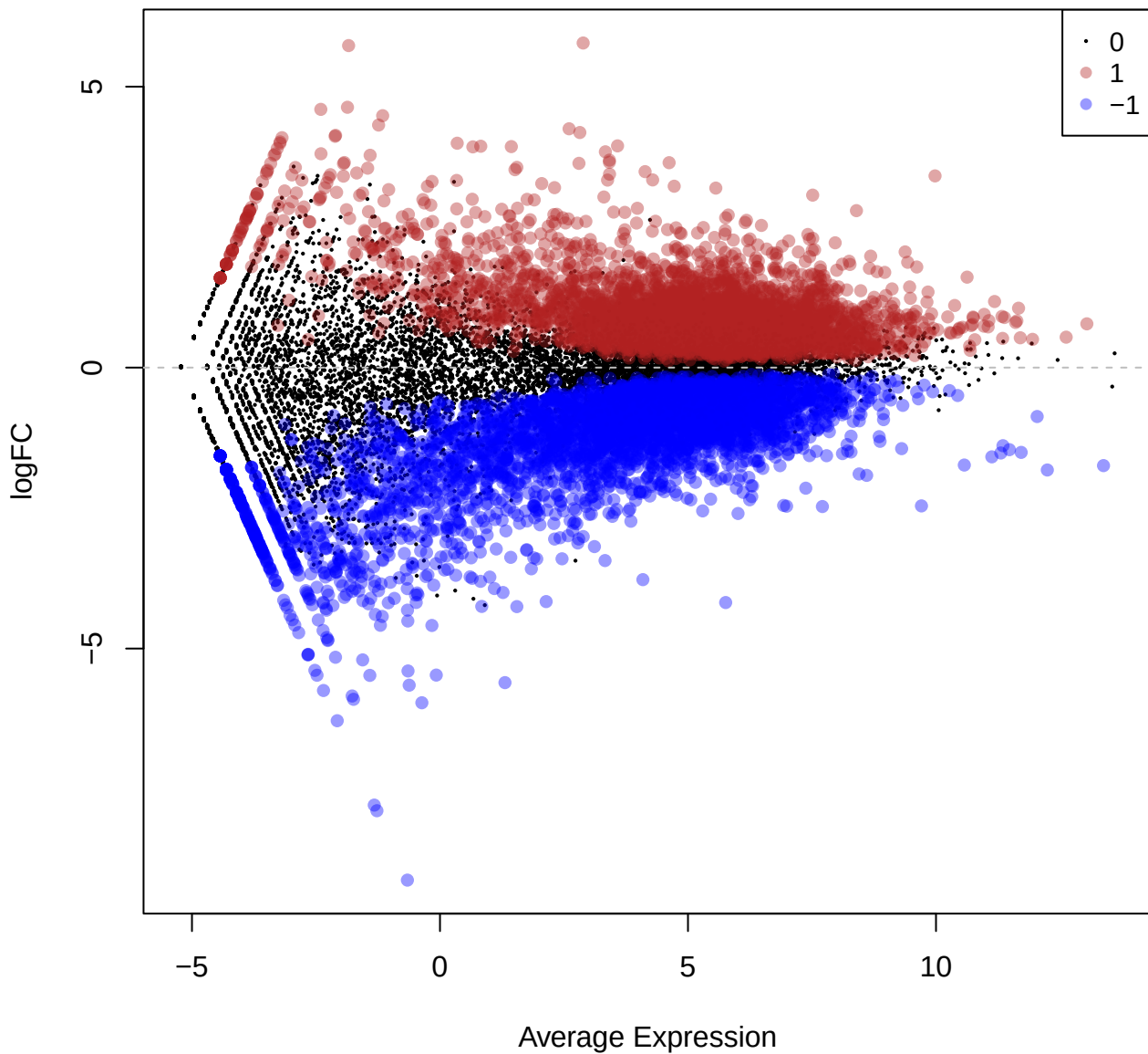
MD Plot: Treated-Control
