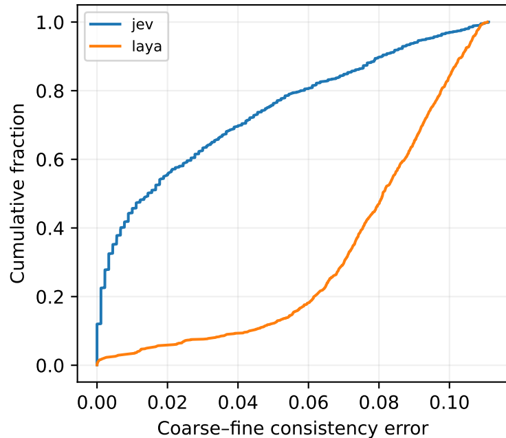
MASSIVE
