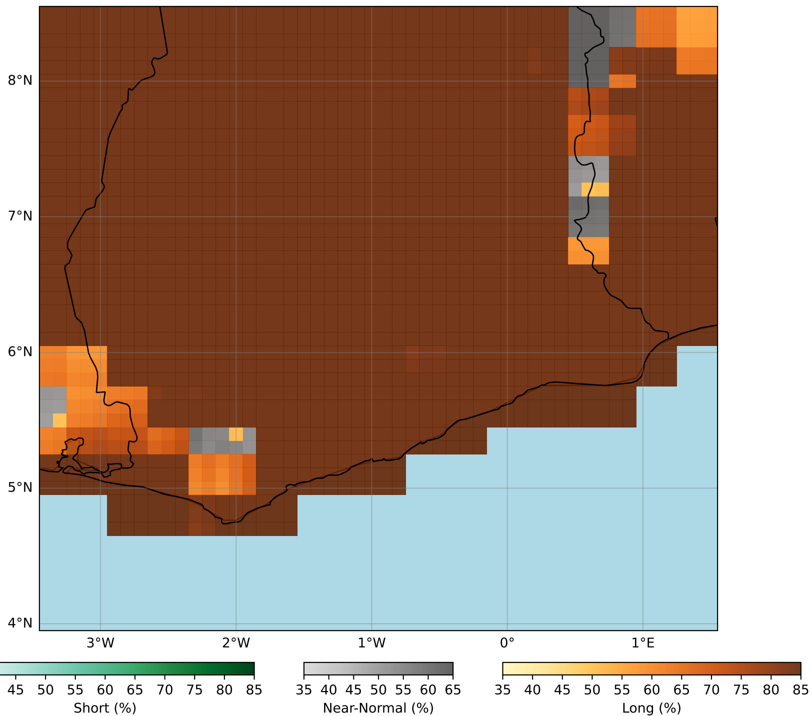
CCA_CMC1_1 dryspellonset-2025 Initial conditions of December
