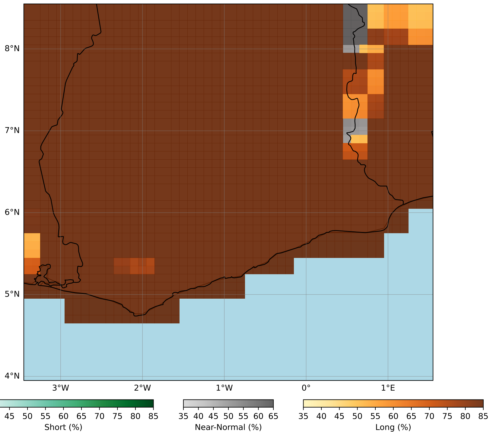
CCA_CMC2_1 dryspellonset-2025 Initial conditions of December
