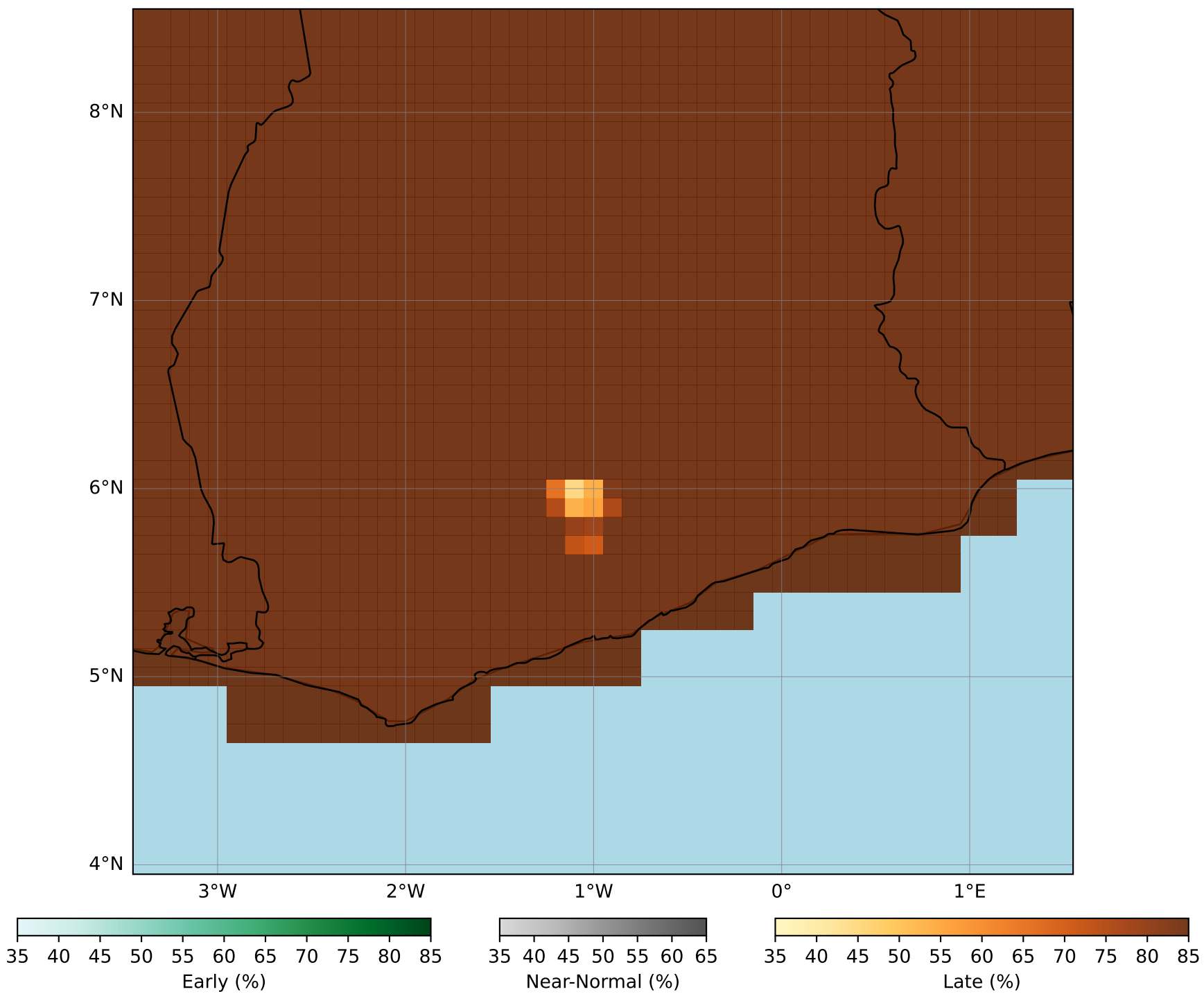
CCA_DWD_22 Onset-2025 Initial conditions of December
