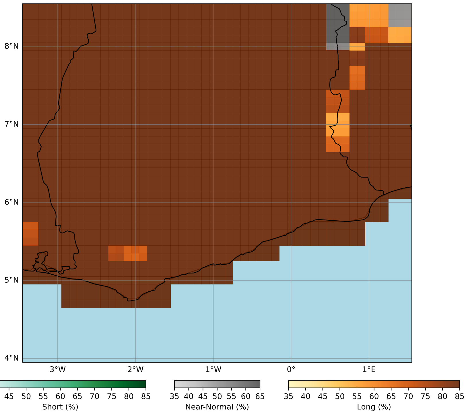
CCA_DWD_22 dryspellonset-2025 Initial conditions of December
