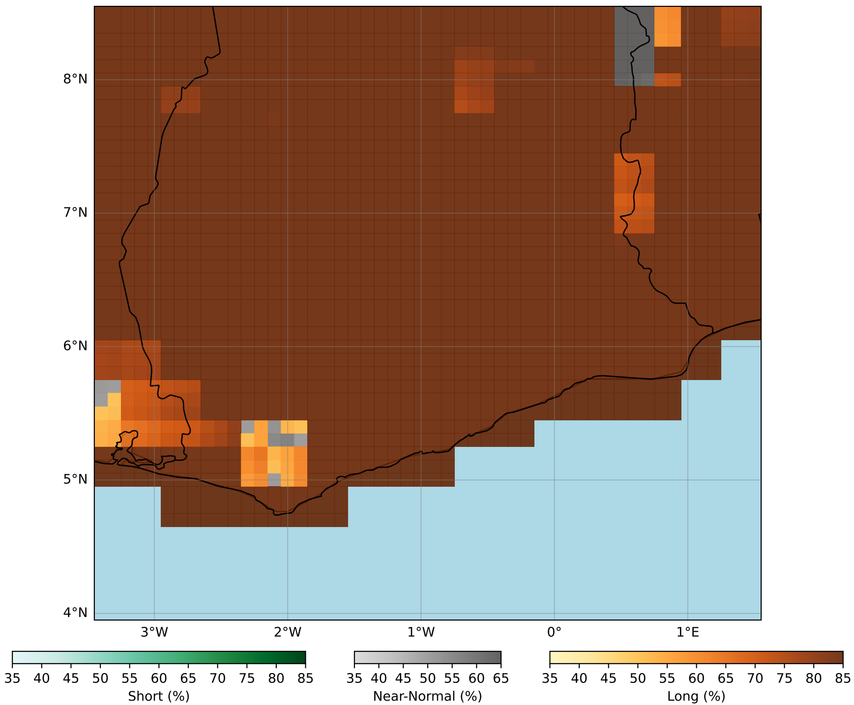
CCA_ECCC_4 dryspellonset-2025Initial conditions of December
