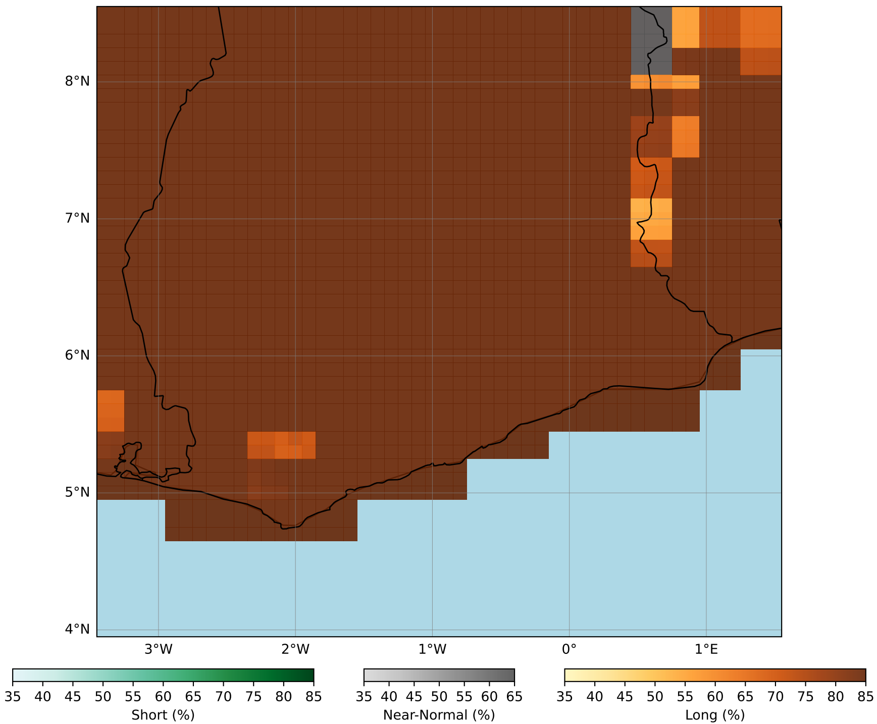
CCA_ECCC_5 dryspellonset-2025Initial conditions of December
