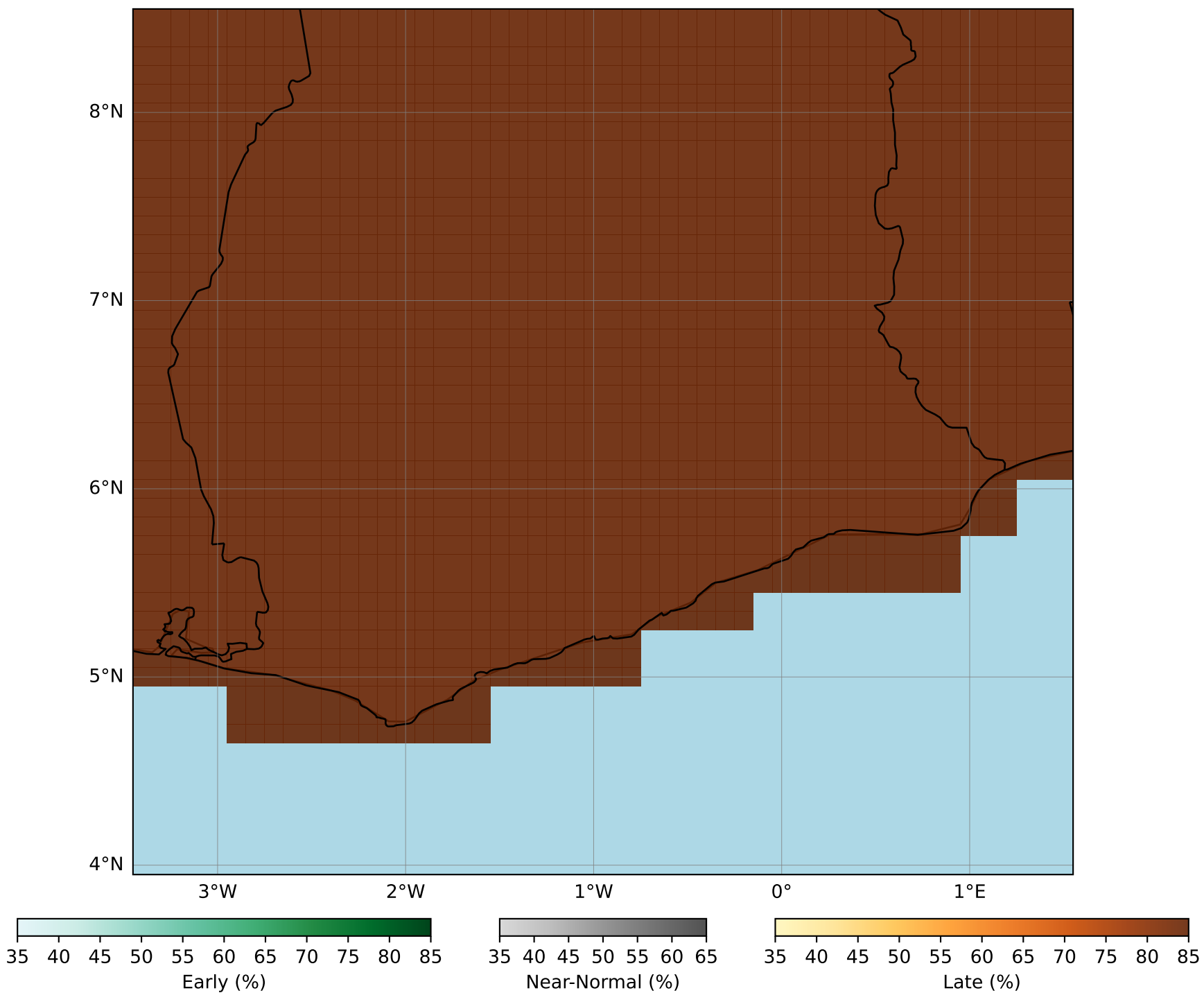
CCA_ECMWF_51 Onset-2025 Initial conditions of December
