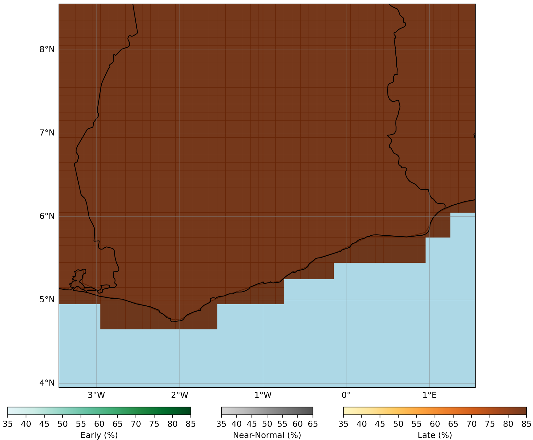
CCA_JMA_3 Onset-2025 Initial conditions of December
