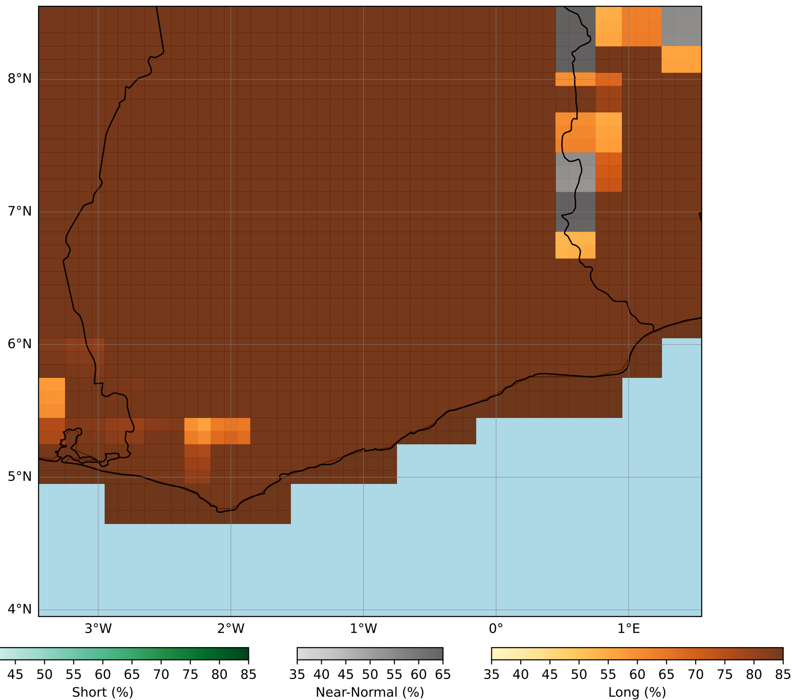
CCA_NCAR_CESM1_1 dryspellonset-2025 Initial conditions of December
