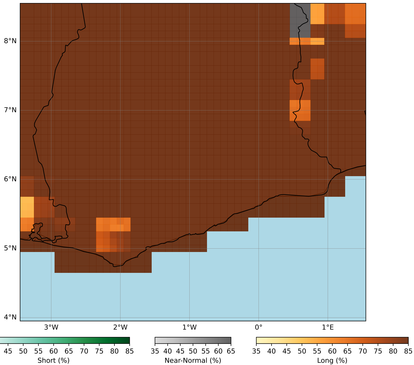
CCA_NCEP_2 dryspellonset-2025Initial conditions of December
