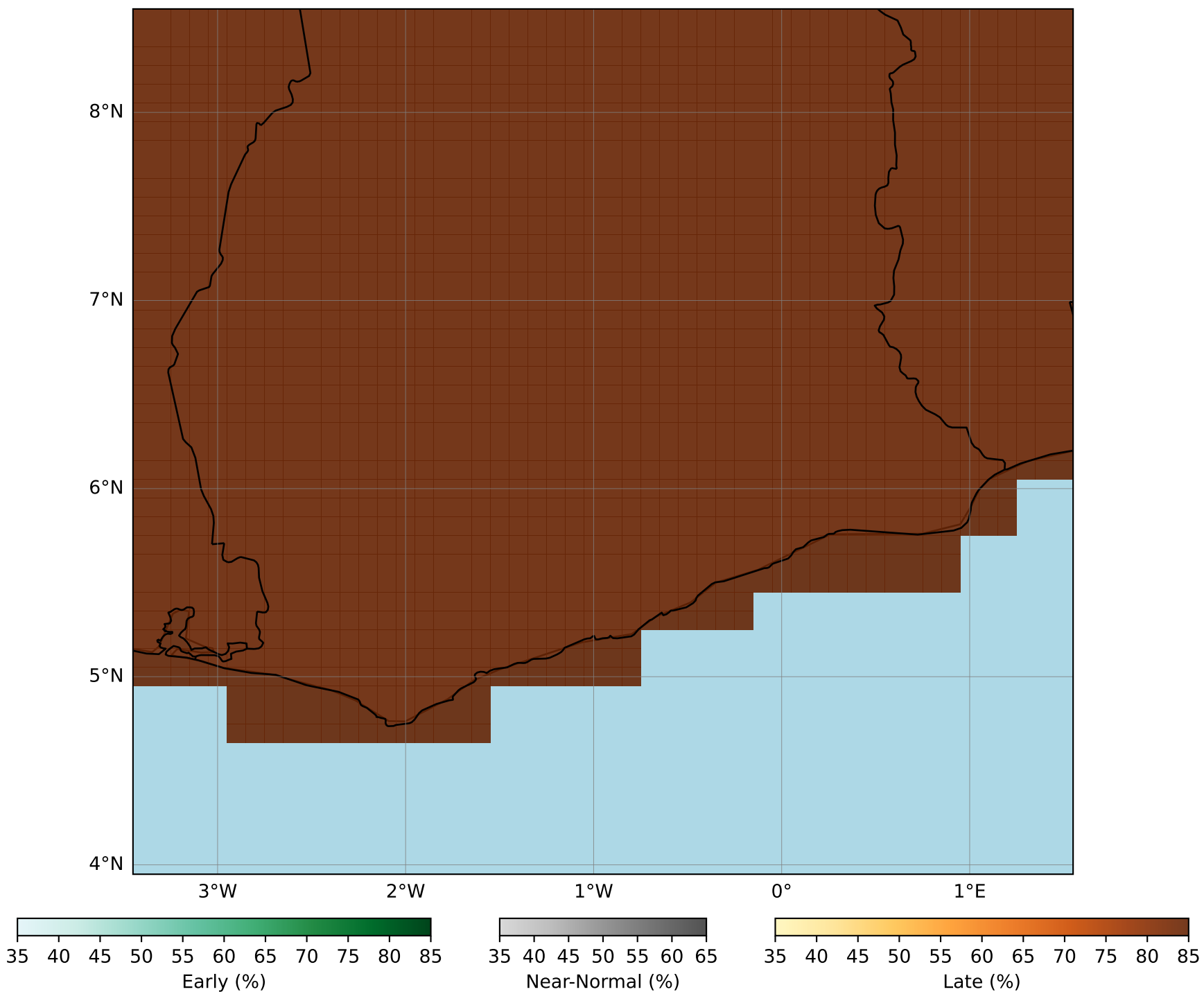
XGBoost Onset-None Initial conditions of December
