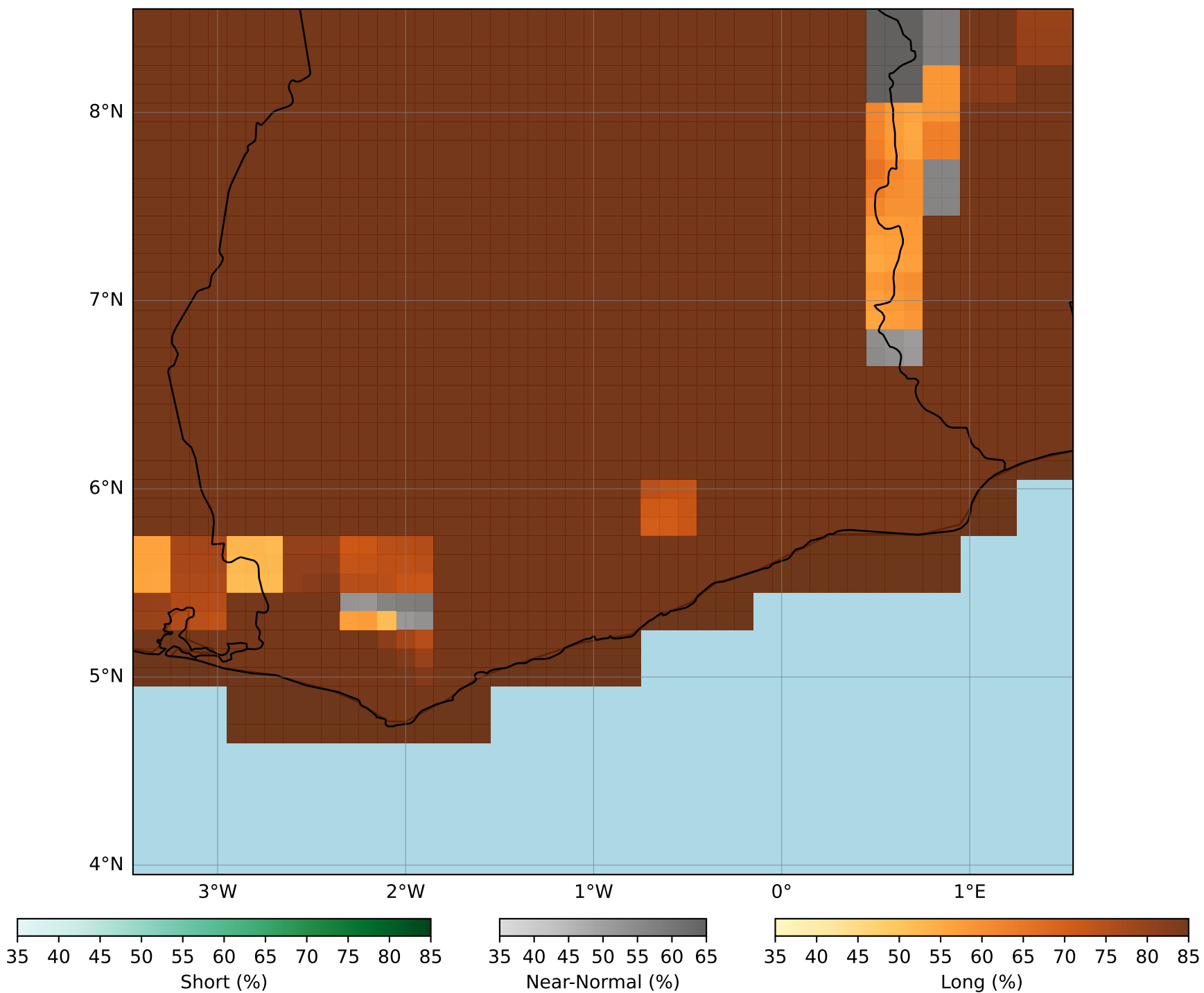
Analogue-Based Forecasting dryspellonset-2025 Initial conditions of December
