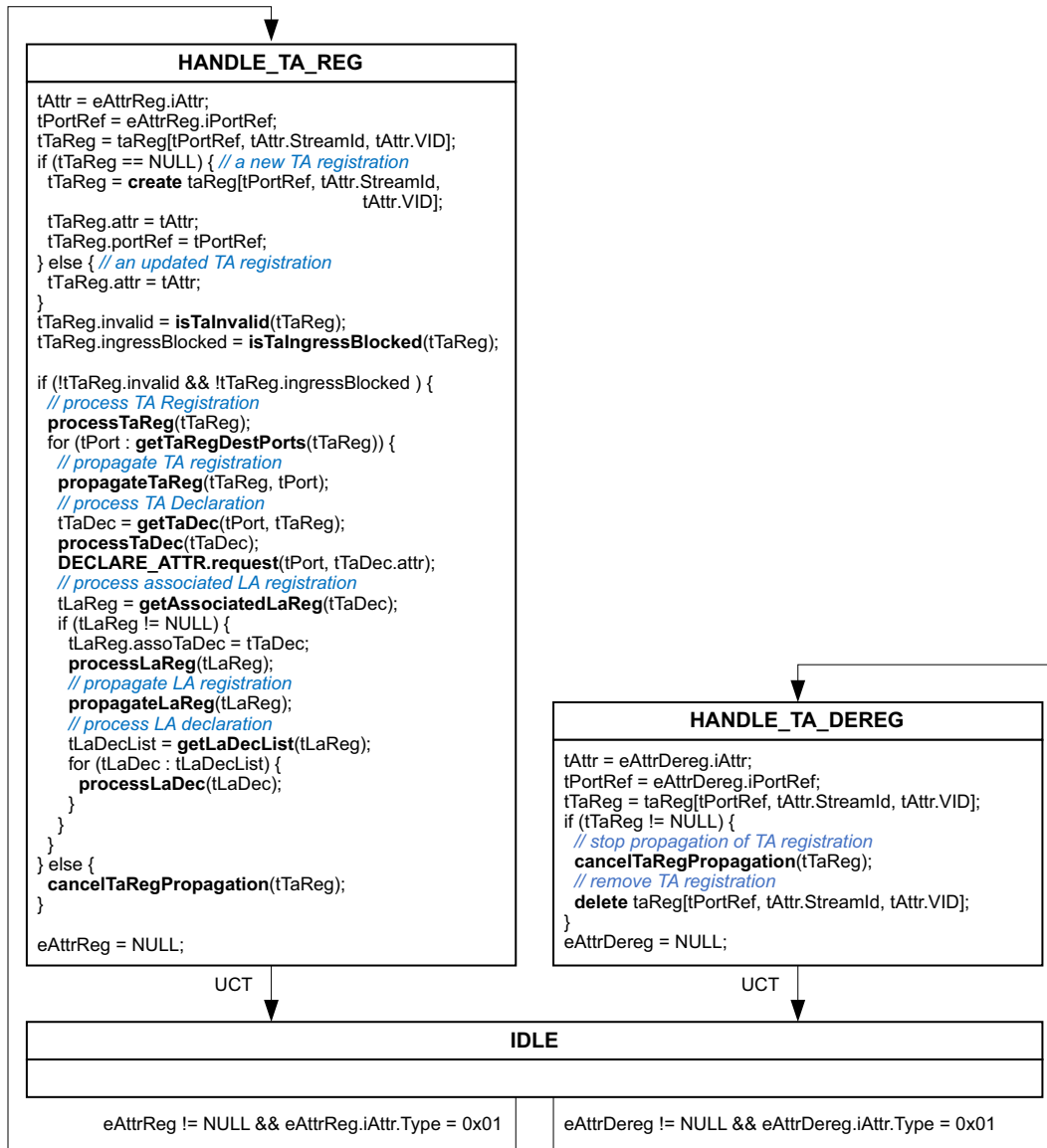
Figure 6-25—Handling of Talker Announce registrations and deregistrations in a RAP Propagator
