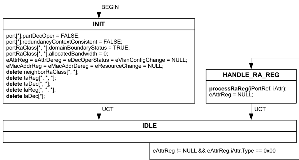
Figure 6-24—Initialization and handling of RA registrations in a RAP Propagator
