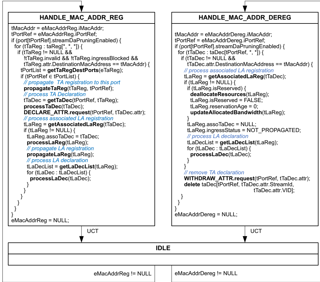
Figure 6-27—Handling of MAC address registrations and deregistrations in a RAP Propagator
