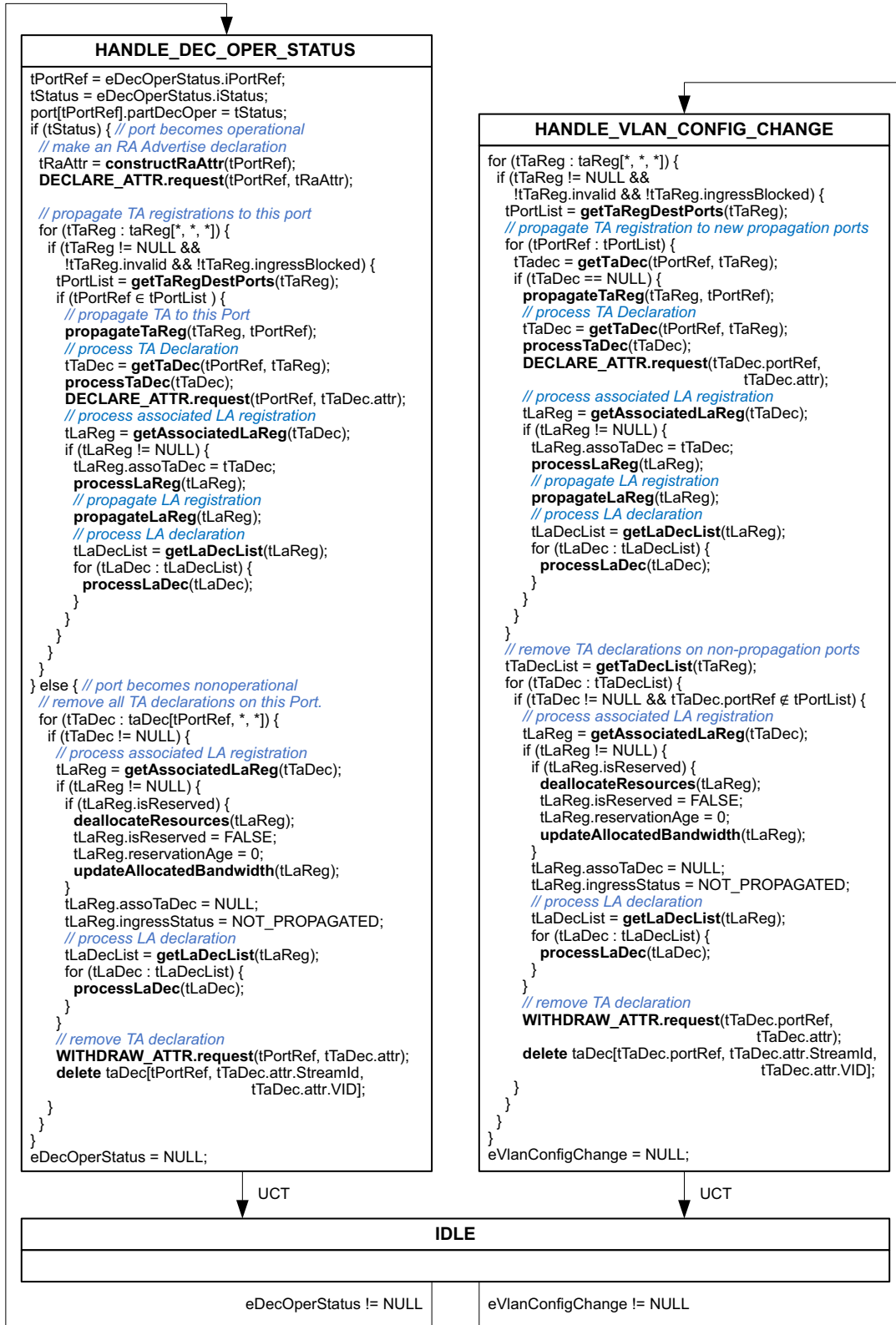
Figure 6-28—Handling of Port status changes and VLAN topology changes in a RAP Propagator
