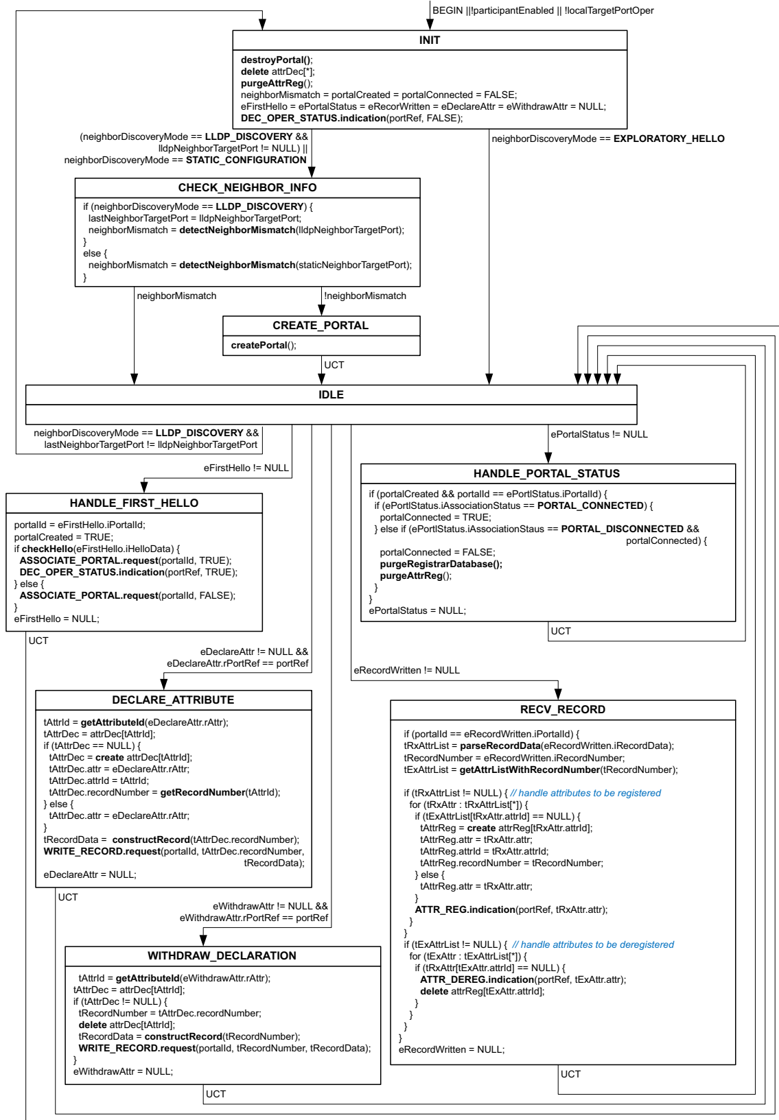
Figure 6-22—RAP Participant state machine diagram
