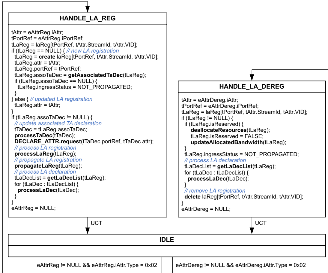
Figure 6-26—Handling of Listener Attach registrations and deregistrations in a RAP Propagator
