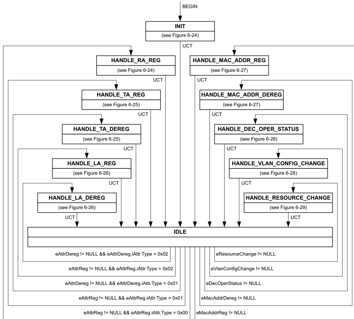
Figure 6-23—RAP Propagator state machine diagram
