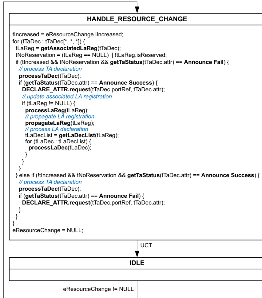
Figure 6-29—Handling of resource availability changes in a RAP Propagator
