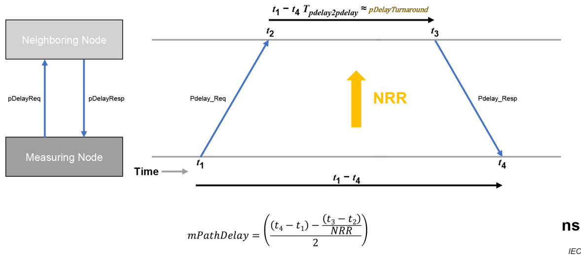
7297 Figure D.8 – Signals and timestamps to measure path delay
