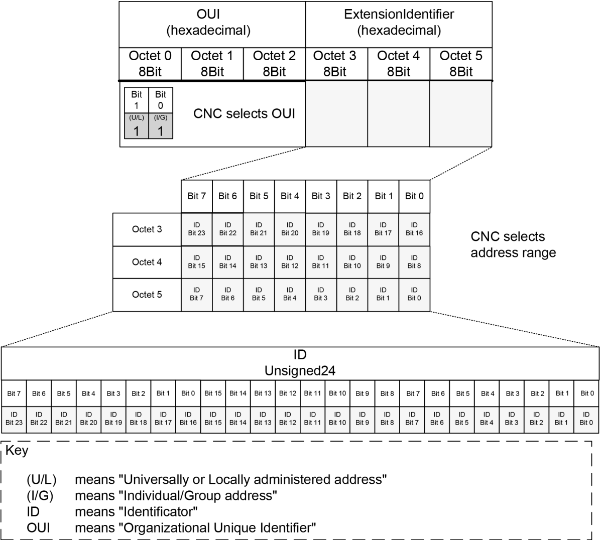
6248 Figure 39 – Stream destination MAC Address
