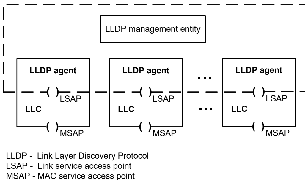
Figure 6-2—Relationship between LLDP agents, LLC Entities, MSAPs, and the LLDP management entity
