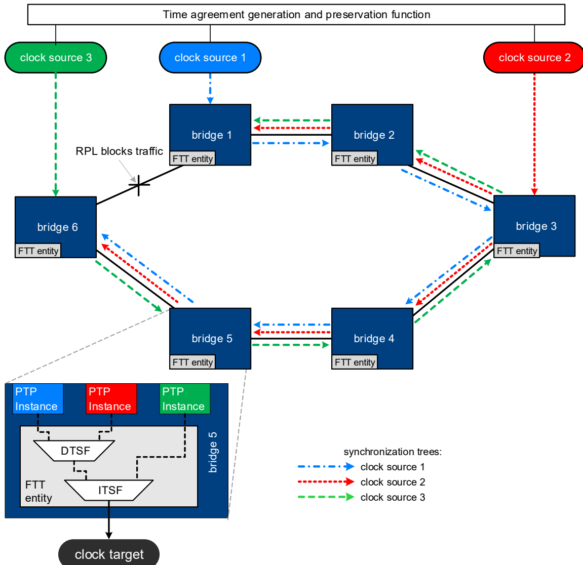
Figure J-6—FTT entity in example ring network
