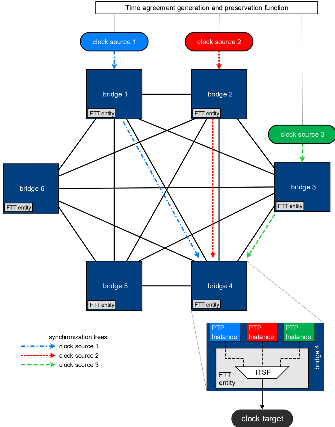
Figure J-8—FTT entity in example mesh network
