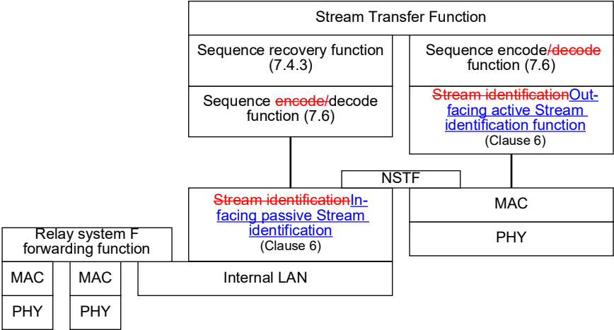
Figure C-7—Protocol stack for relay system F in Figure C-4
