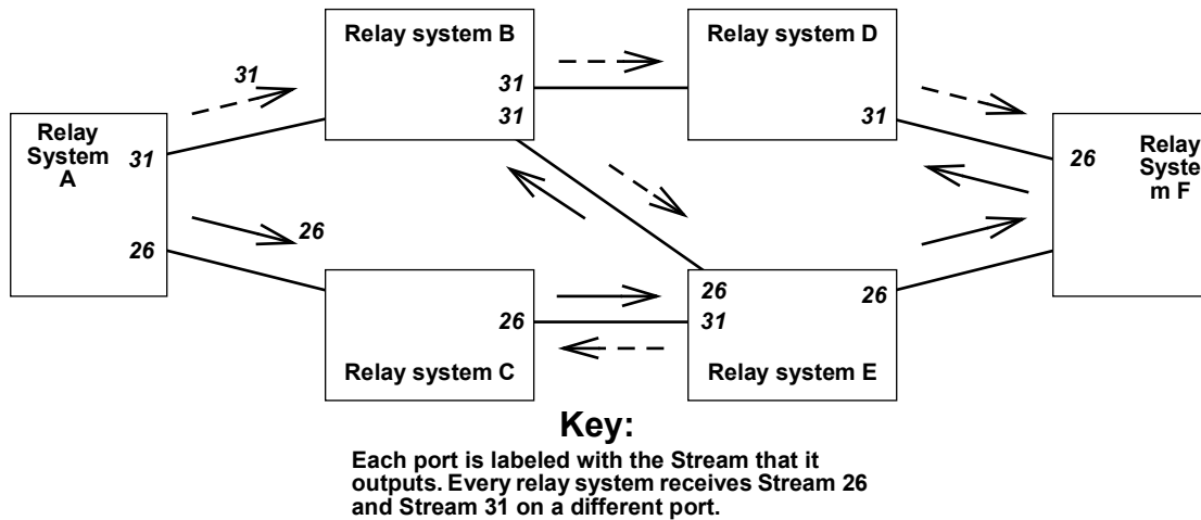
Figure C-9—Multicast trees
