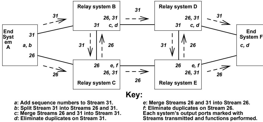
Figure C-8—Ladder redundancy
