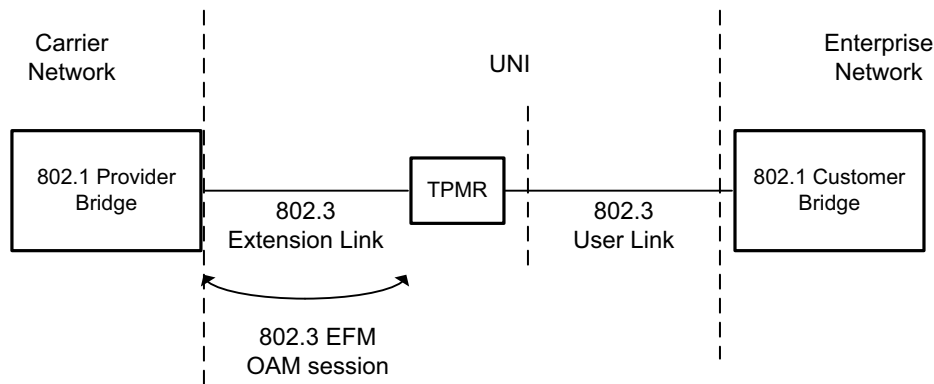
Figure K-1—TPMR as UNI demarcation device
