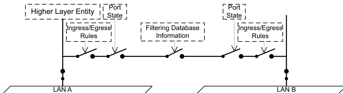
Figure 8-30—Ingress/egress control information in the forwarding path
