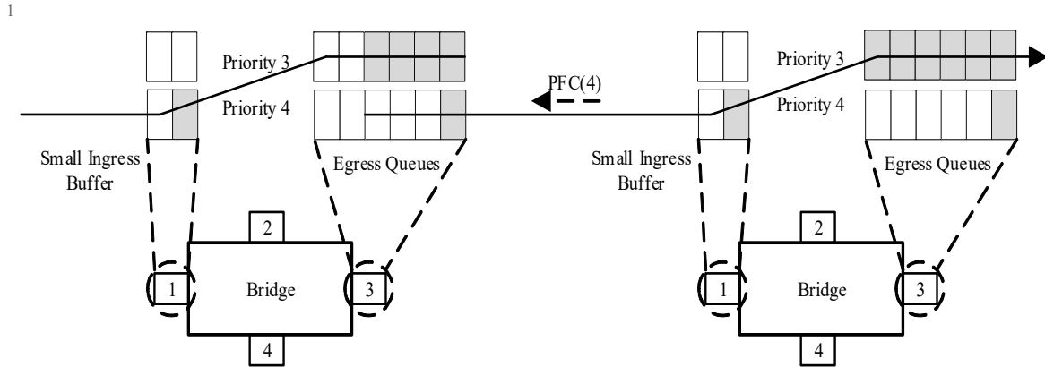
Figure W-9—Example PFC request to avoid packet loss with CI enabled
