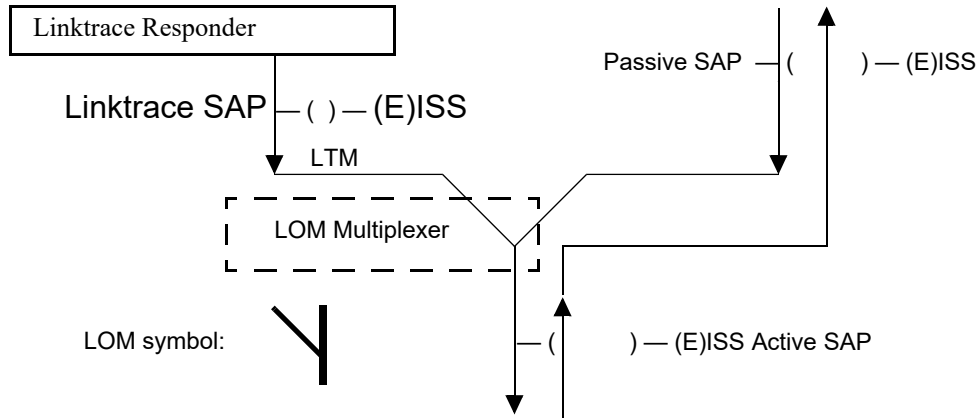
Figure 19-5—LOM architecture
