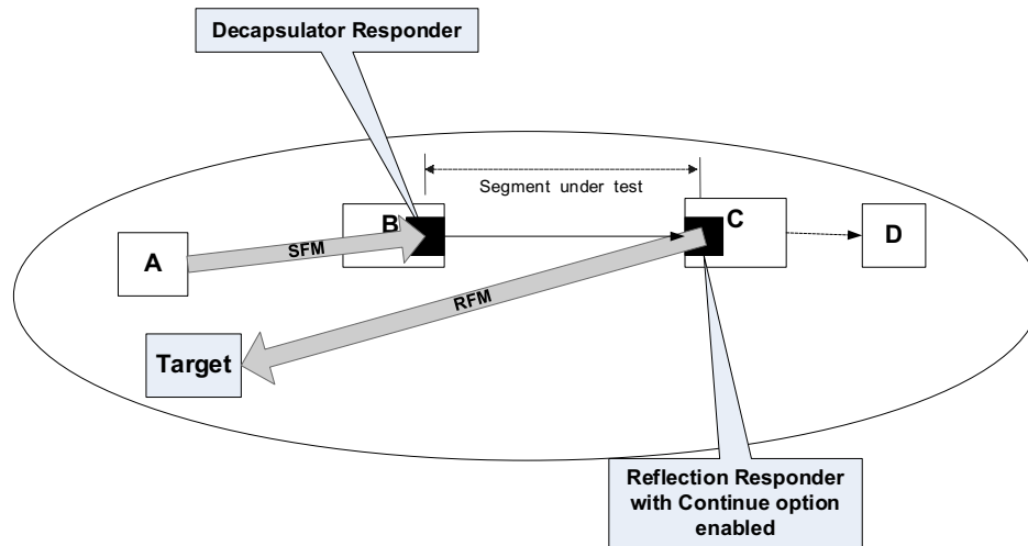
Figure 29-3—Combination of FPT and RPT
