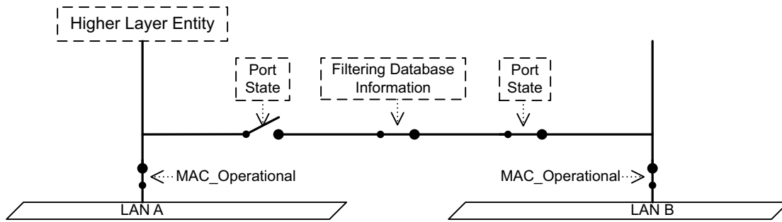
Figure 8-27—Single point of attachment—relay not permitted
