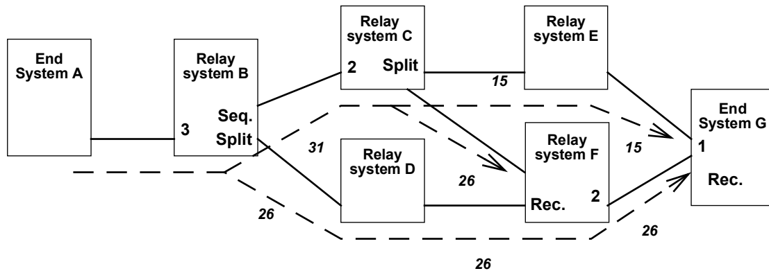
Figure C-4—Frame Replication and Elimination for Reliability RER flexible positioning
