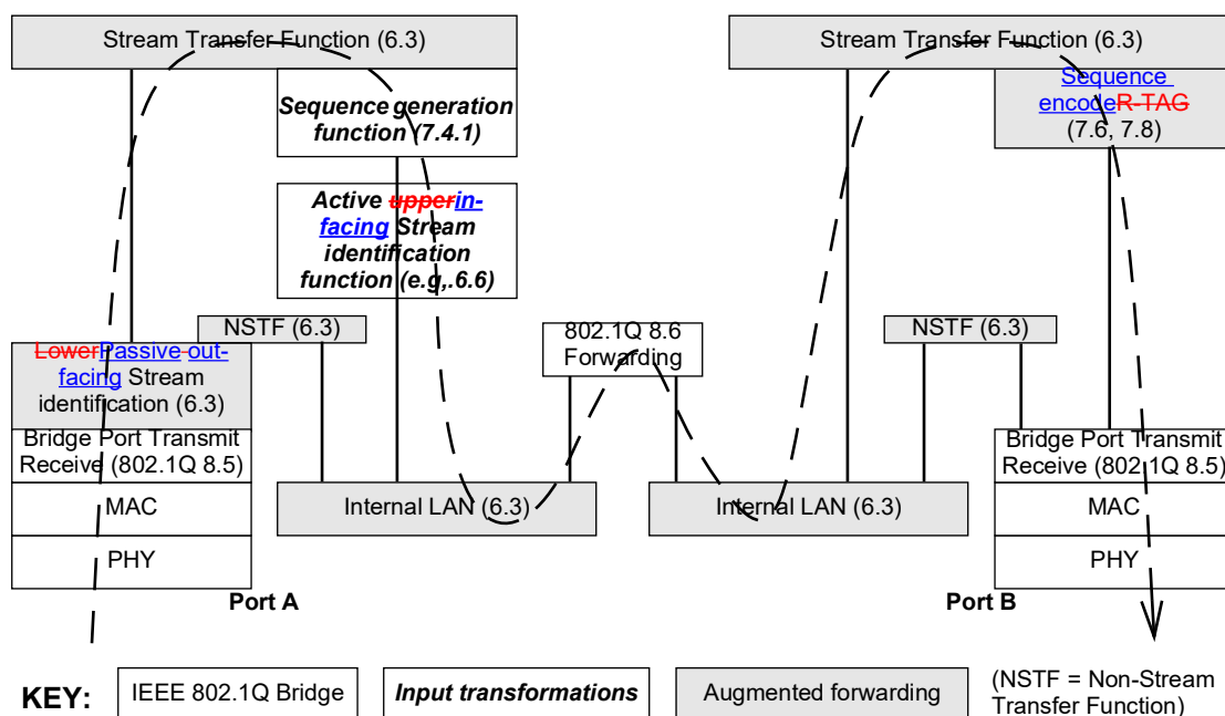
Figure 8-1—Split functions in an FRER C-component
