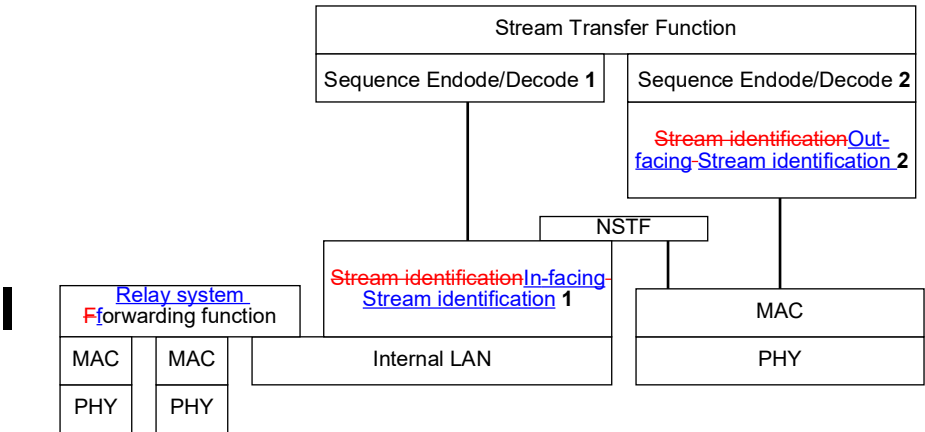
Figure C-10—Protocol interworking
