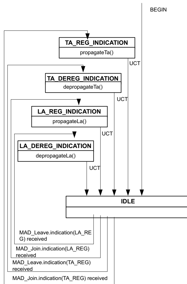
Figure 6-23—RAP MAP state machine
