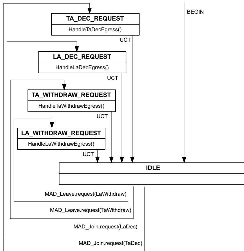
Figure 6-20—RAP MAD egress state machine
