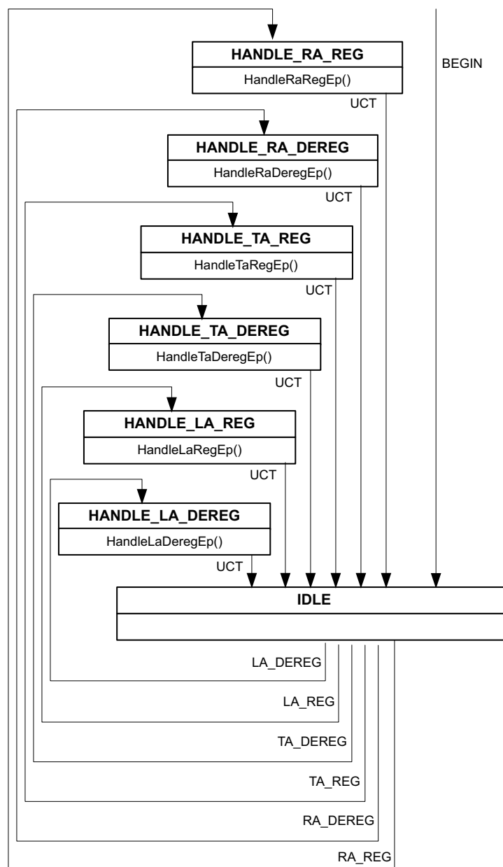
Figure 6-22—RAP Endpoint state machine
