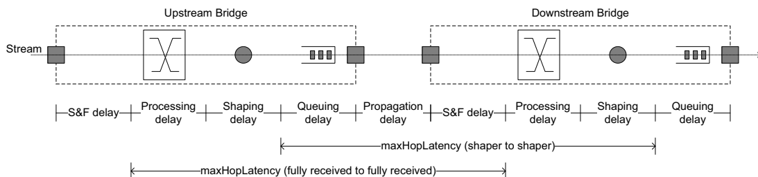
Figure 6-3—Latency reference points
