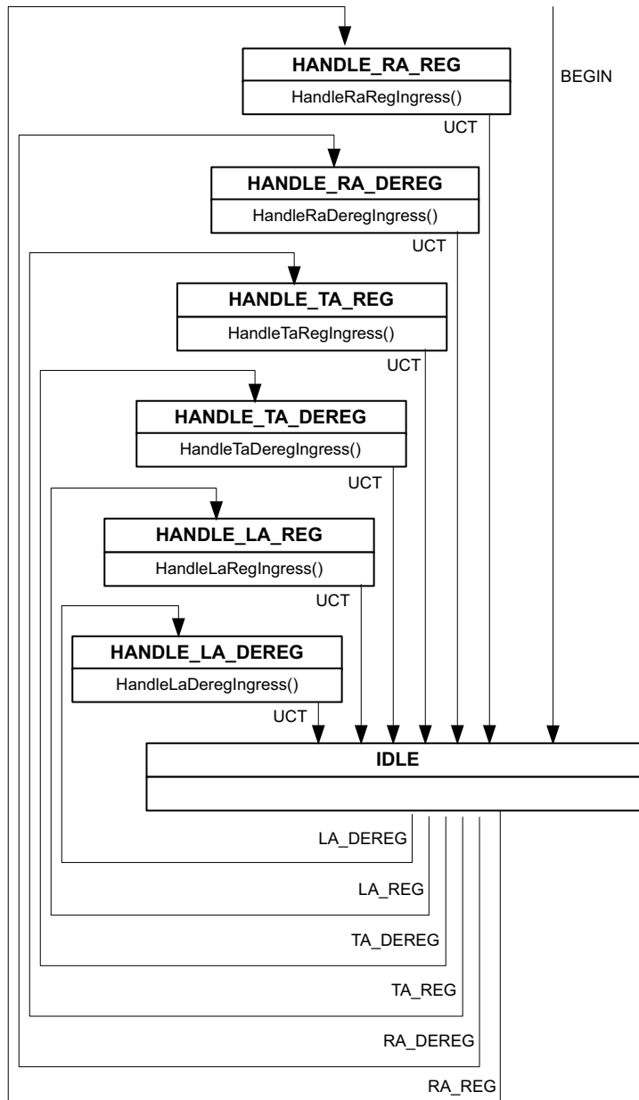
Figure 6-19—RAP MAD ingress state machine
