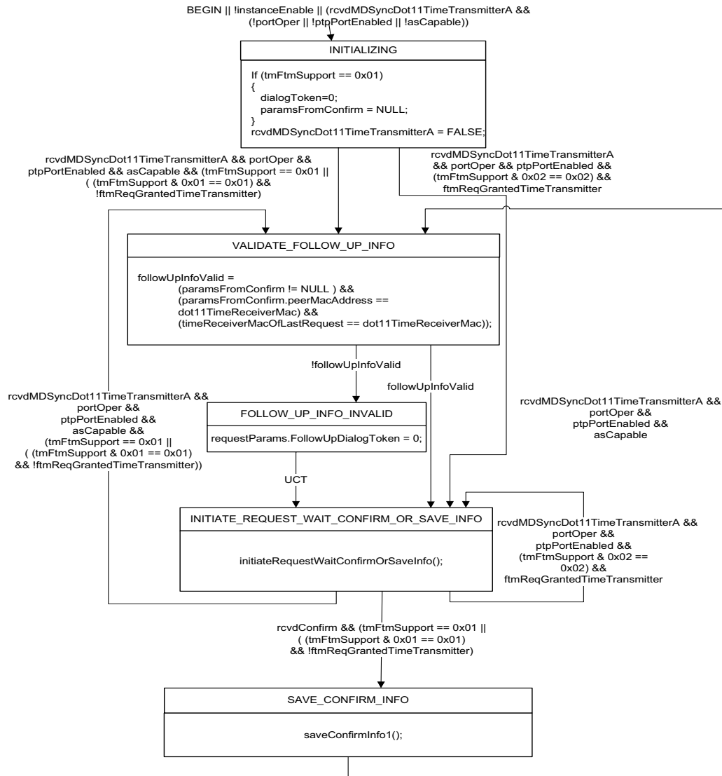
Figure 12-5—TimeTransmitter state machine A
