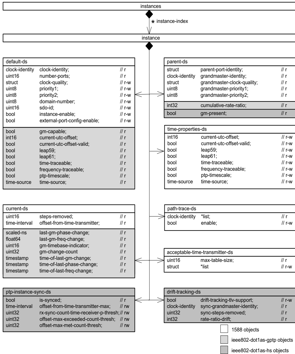
Figure 17-2—PTP Instance detail
