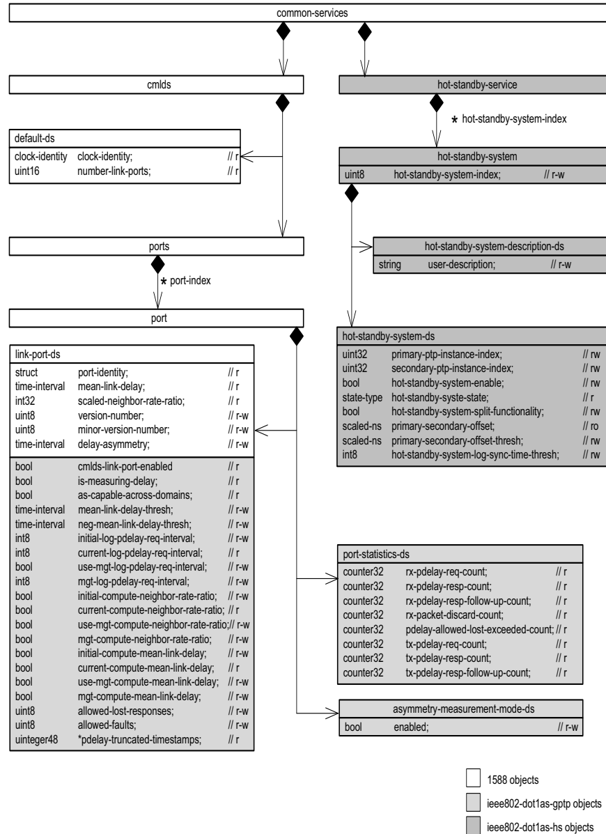
Figure 17-4—Common services detail
