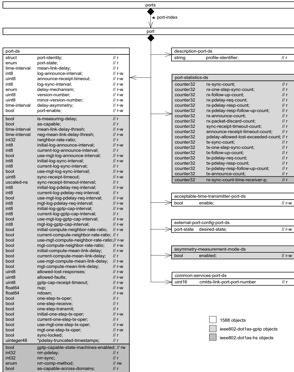
Figure 17-3—PTP Port detail
