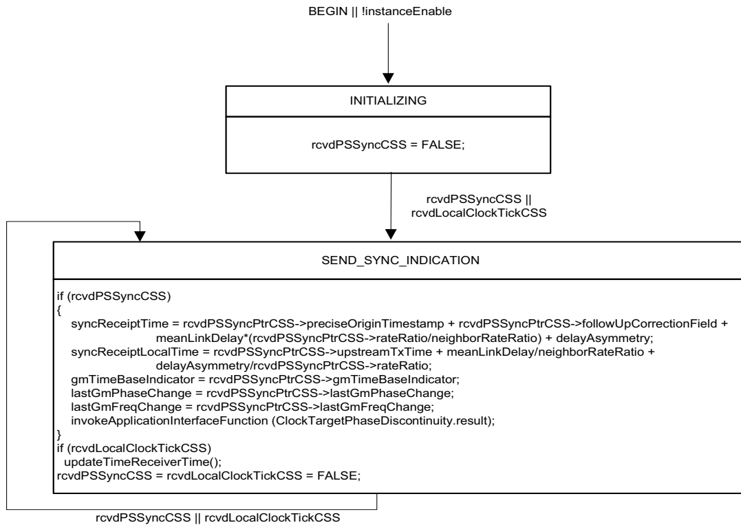
Figure 10-9—ClockTimeReceiverSync state machine
