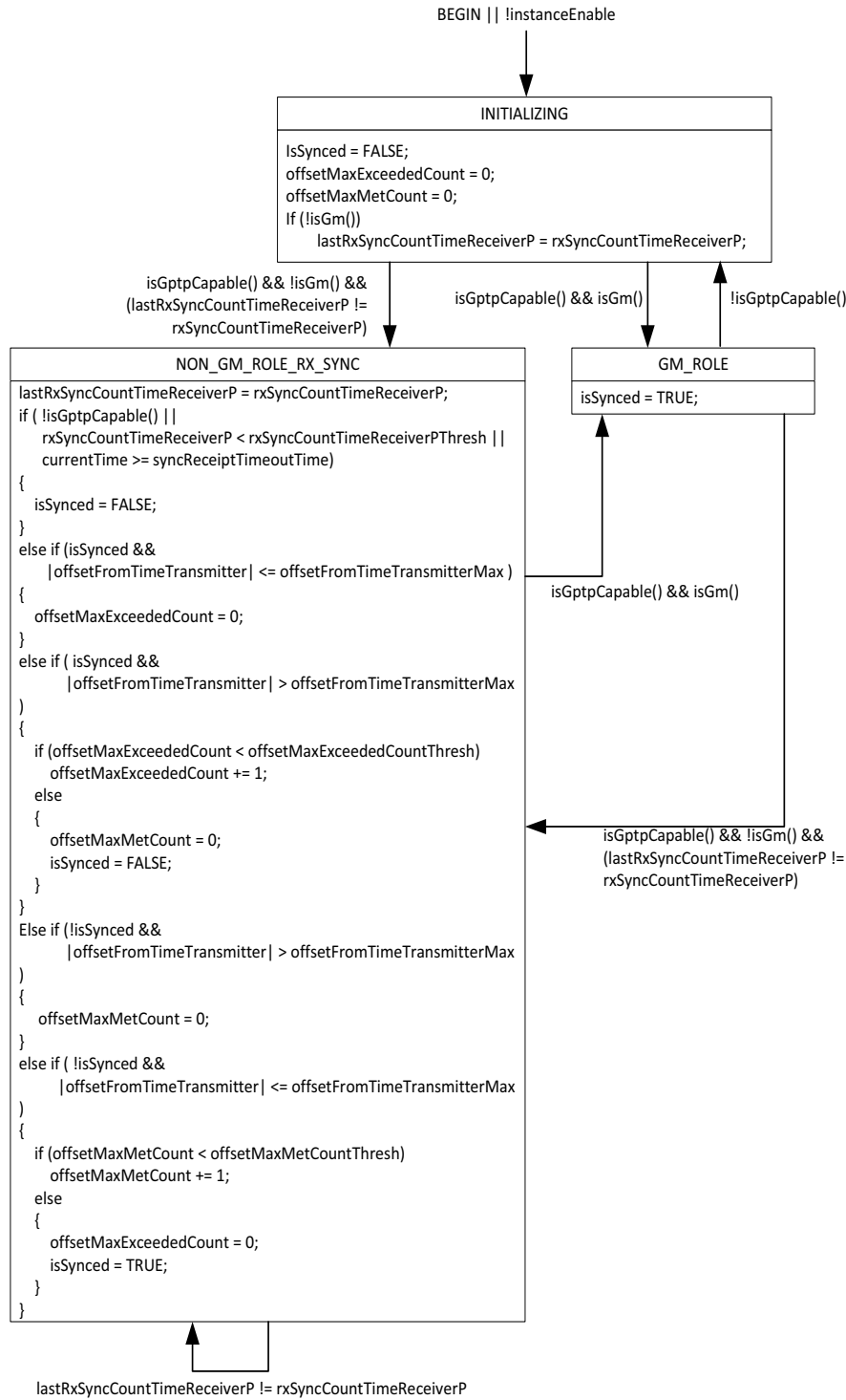
Figure 18-2—PtpInstanceSyncStatus state machine
