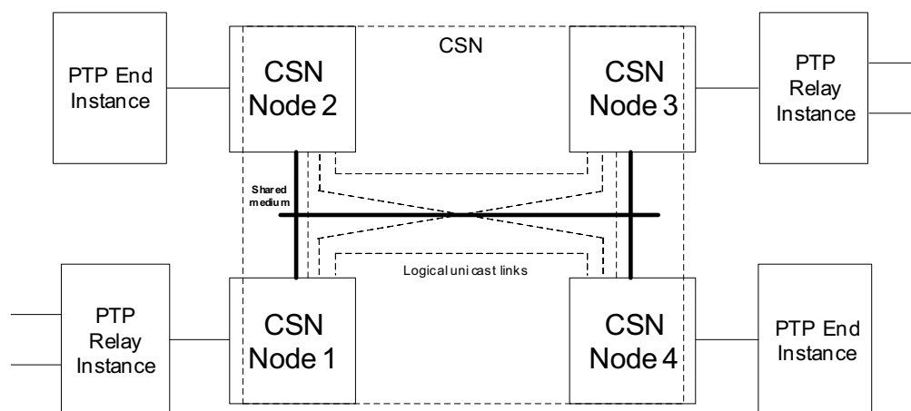
Figure 16-1—Example of CSN backbone
