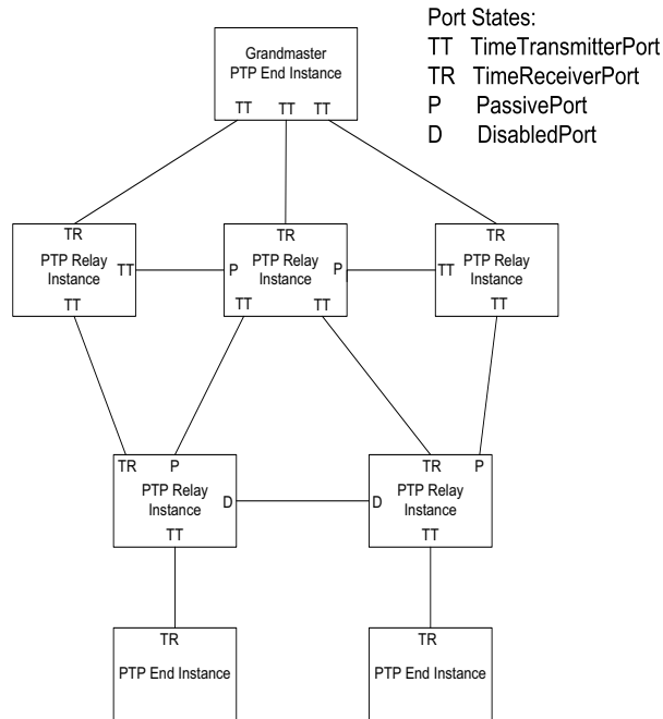
Figure 10-10—Example timeTransmitter/timeReceiver hierarchy of PTP Instances
