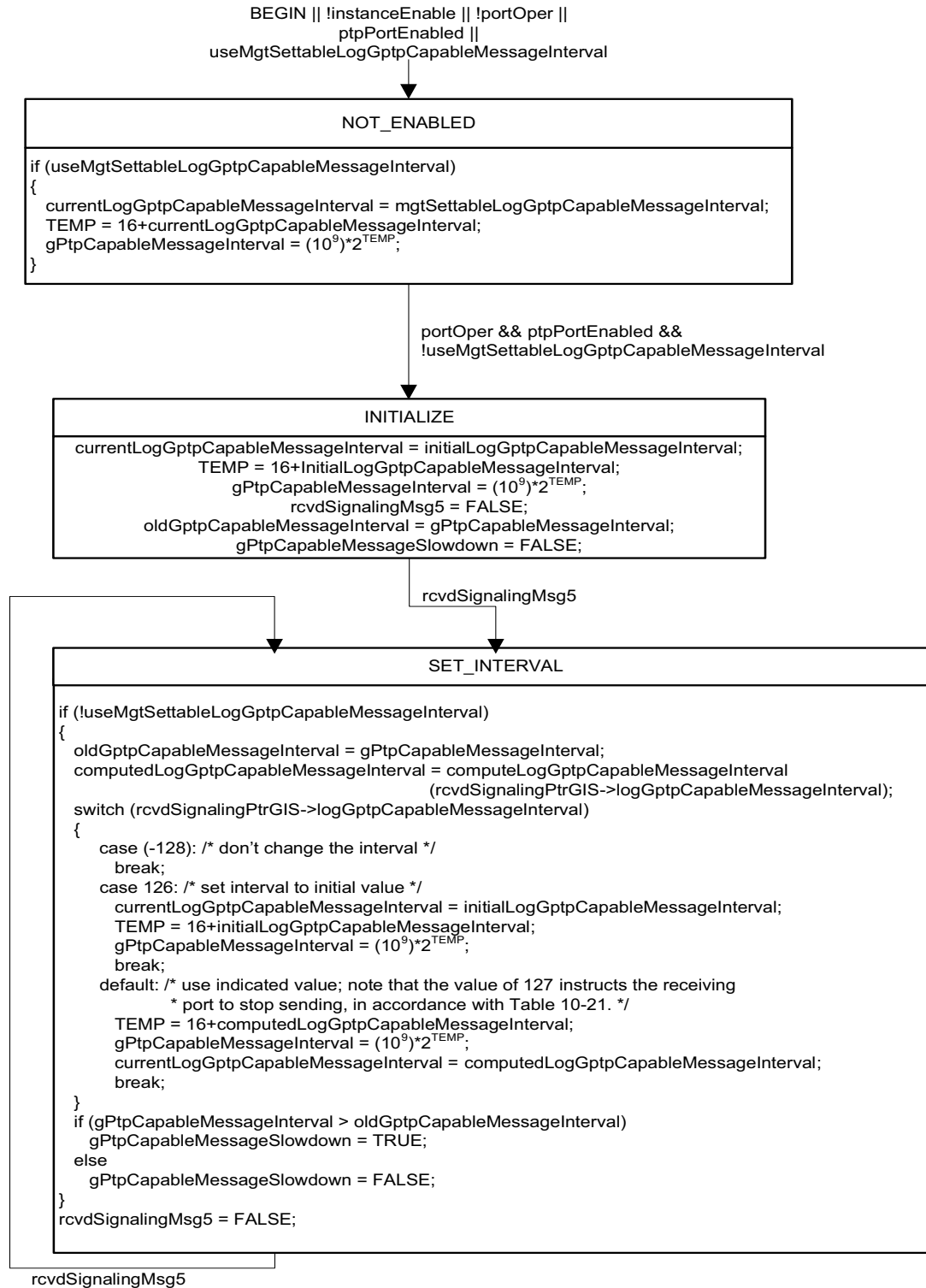
Figure 10-23—GtpCapableIntervalSetting state machine
