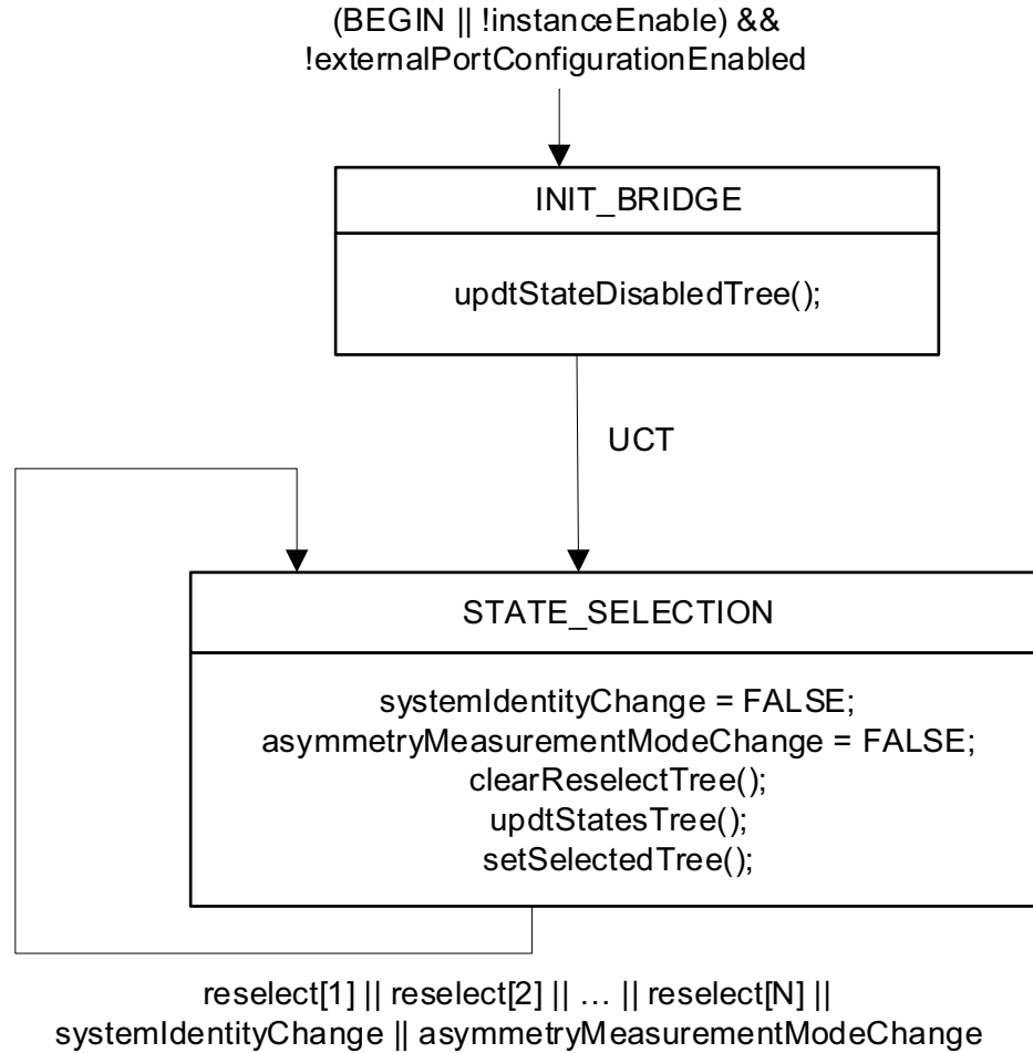
Figure 10-15—PortStateSelection state machine
