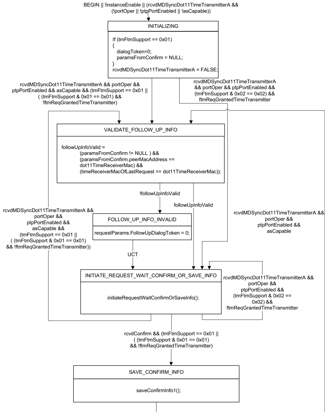
Figure 12-5—TimeTransmitter state machine A (a) For TM, receives information from the PortSync entity and sends to timeReceiver, and (b) For FTM, receives and stores information from the PortSync entity
