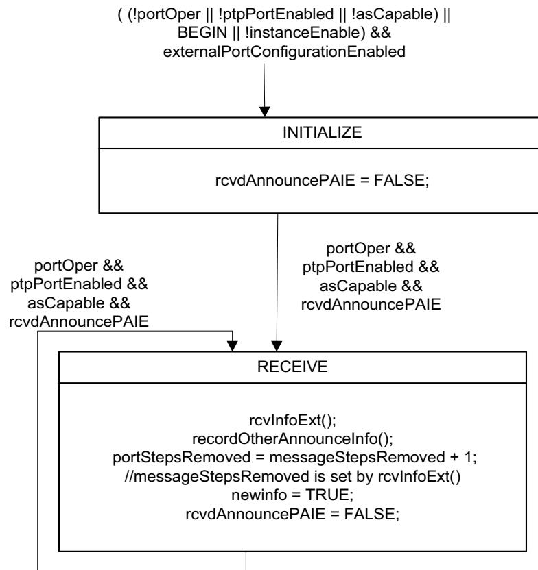
Figure 10-16—PortAnnounceInformationExt state machine
