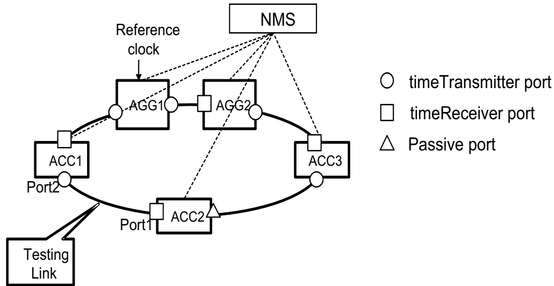
Figure G-1—Asymmetry Compensation Measurement Procedure
