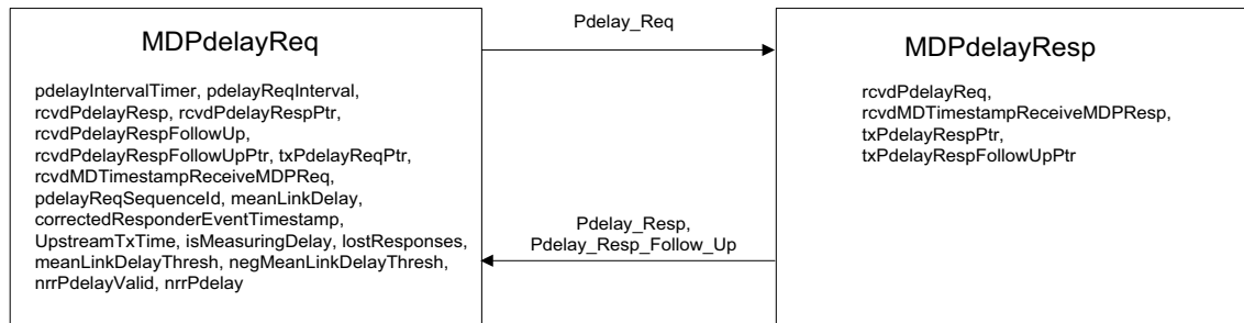
Figure 11-5—Peer-to-peer delay mechanism state machines—overview and interrelationships
