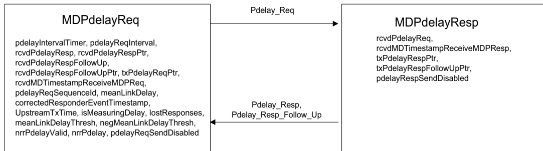
Figure 11-5—Peer-to-peer delay mechanism state machines—overview and interrelationships
