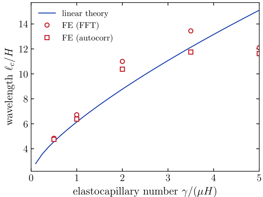
Wrinkle wavelength
