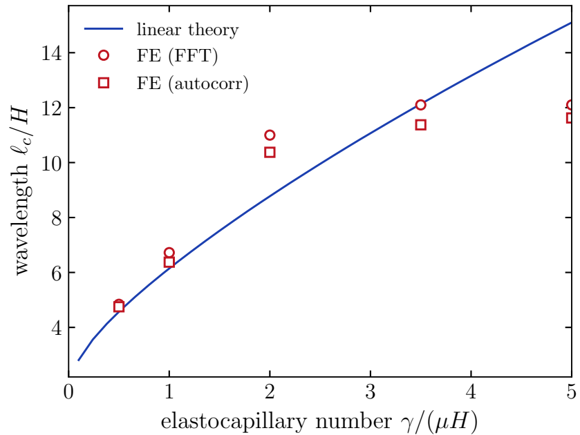
Wrinkle wavelength
