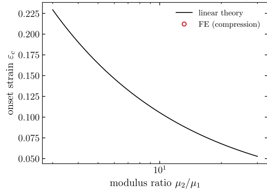
Onset strain (film/substrate, H_1=8, H_2=1 )
